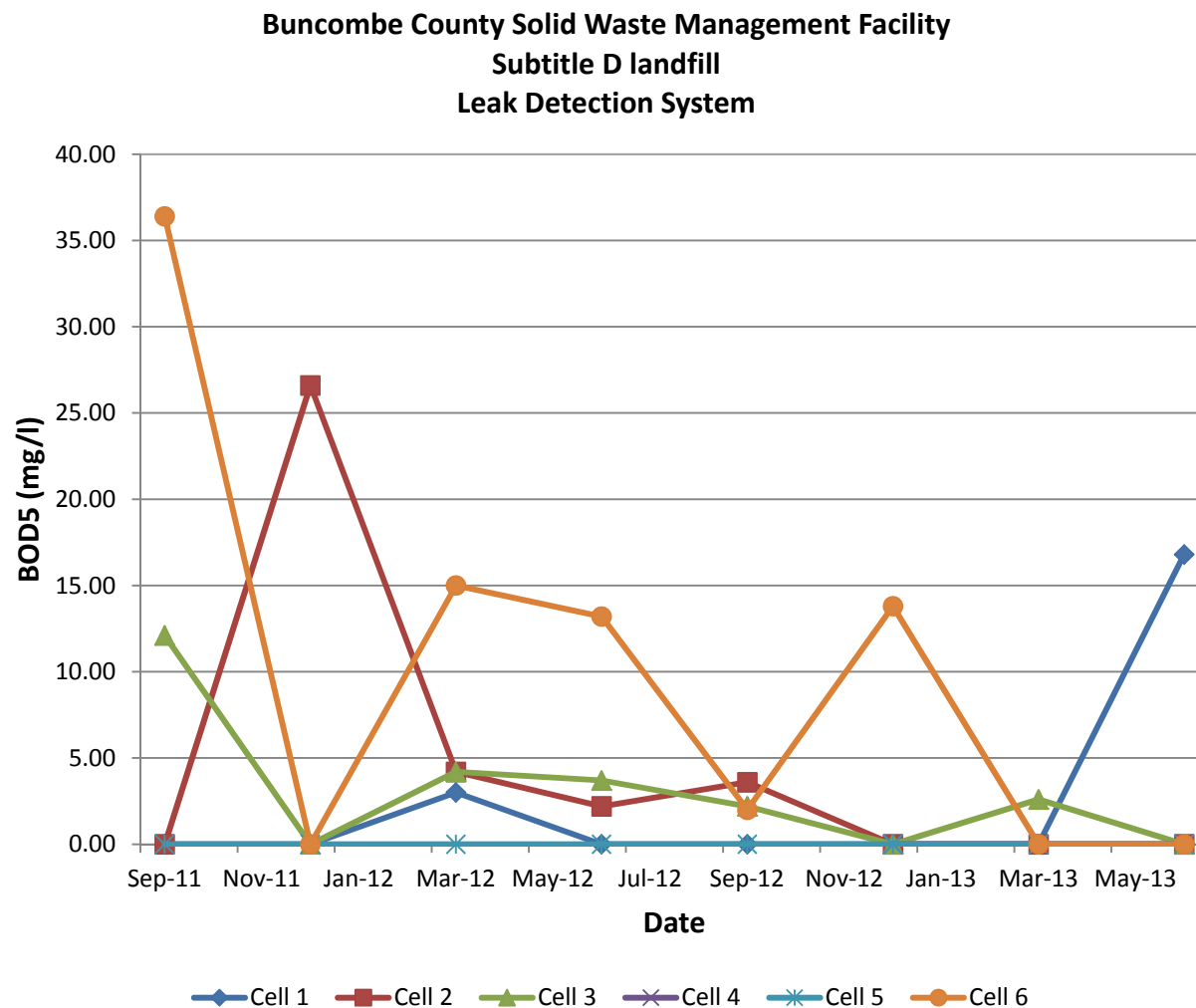
Figure 4-5 BOD5
