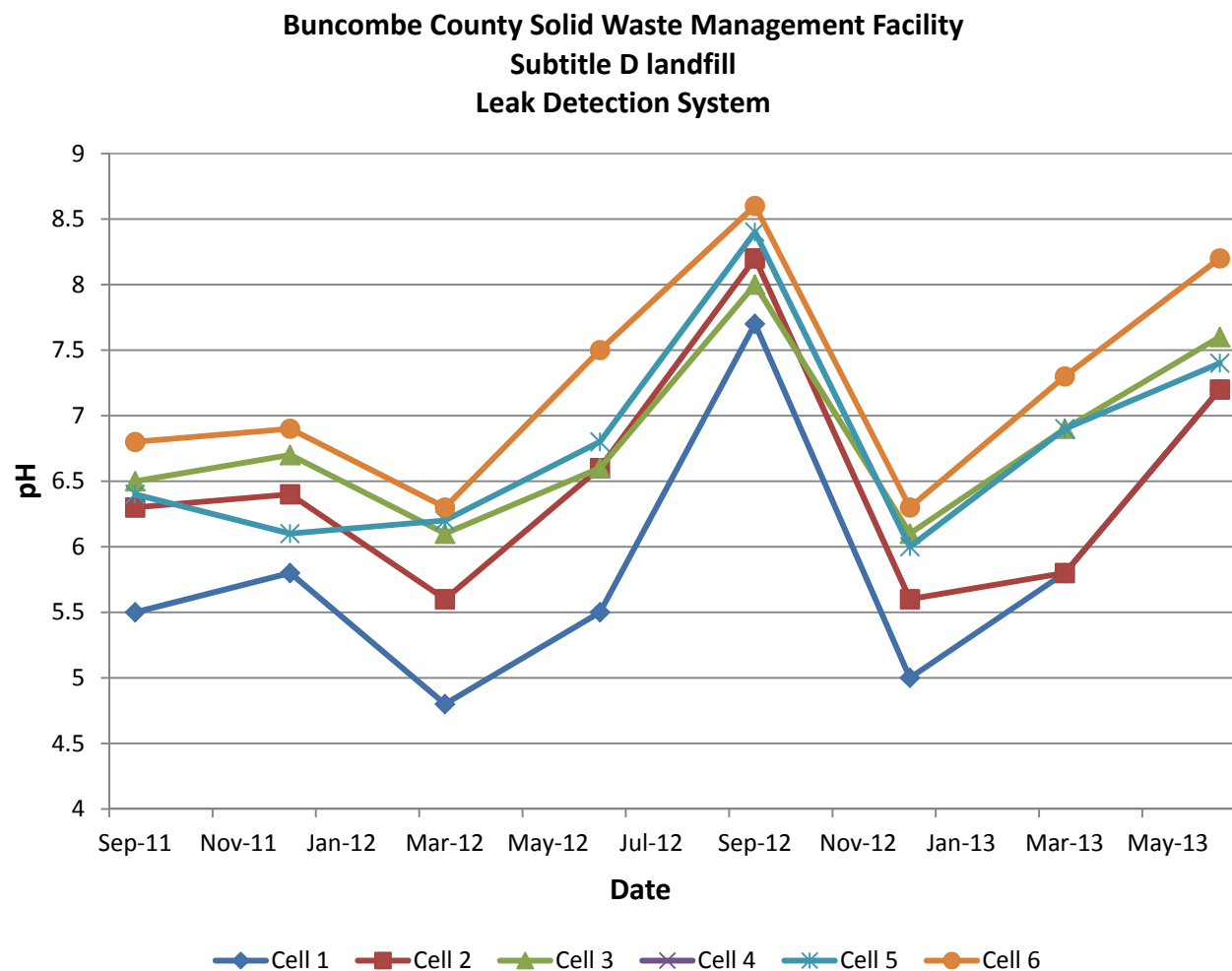
Figure 4-2 pH
