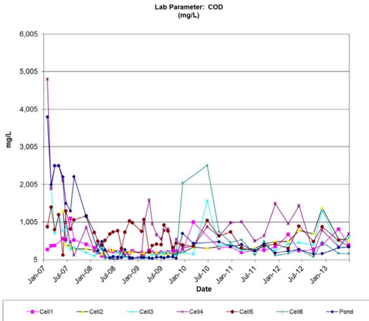
Figure 4-10 COD of Leachate
