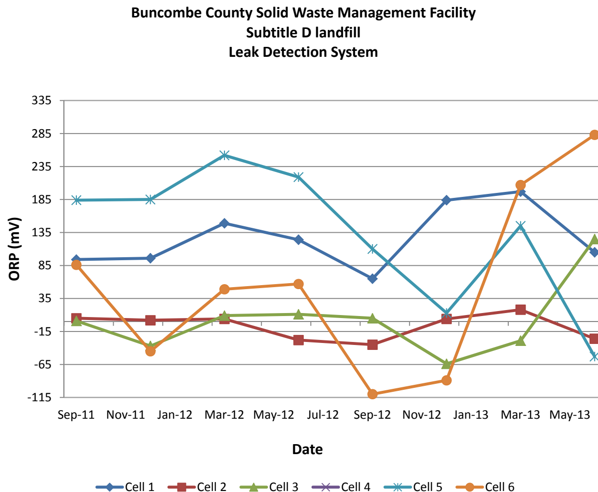
Figure 4-4 Oxidation Reduction Potential
