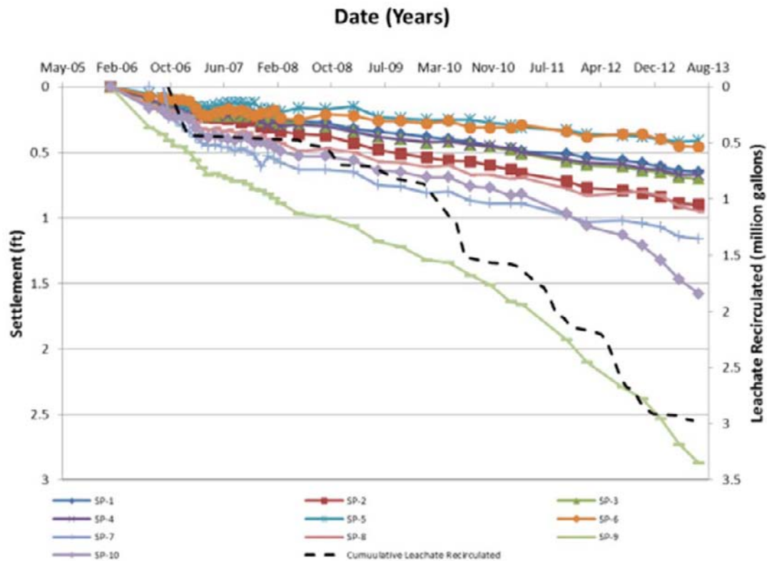
Figure 4-18 Cumulative Settlement
