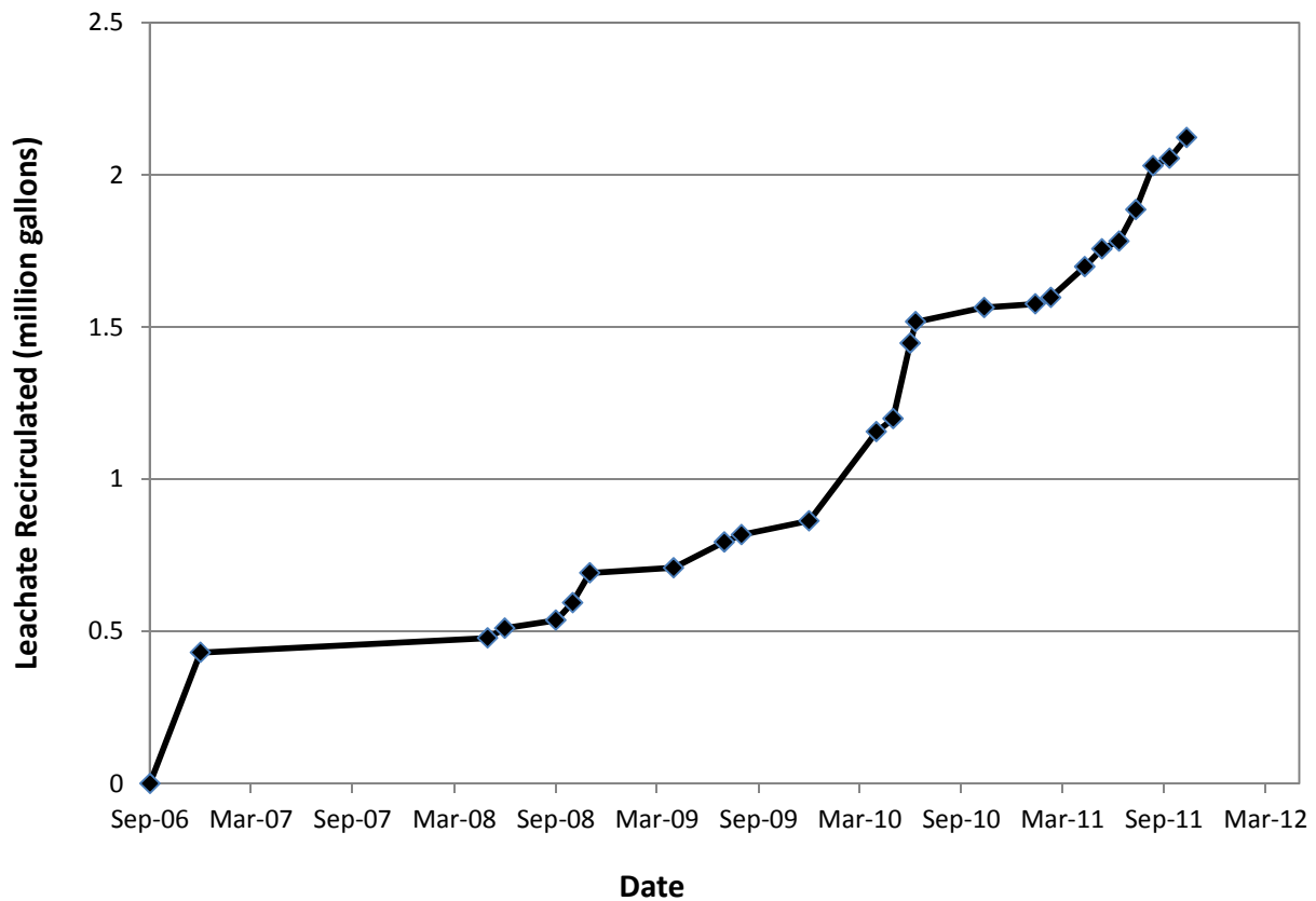
Figure 4-15 – Cumulative Volume of Leachate Recirculated
