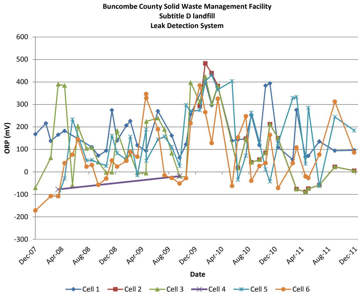
Figure 4-6 – Oxidation Reduction Potential of Liquids for Cells 1-6 in Leak Detection Zone
