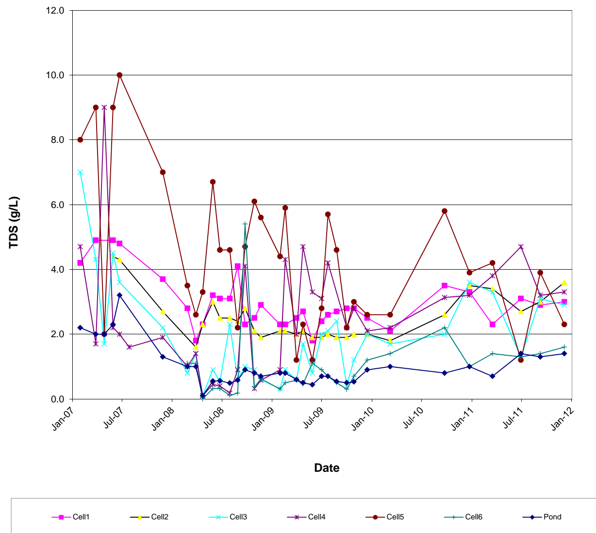
Figure 4-14 – TDS of Leachate from Cells 1-6 and Pond in LCS
