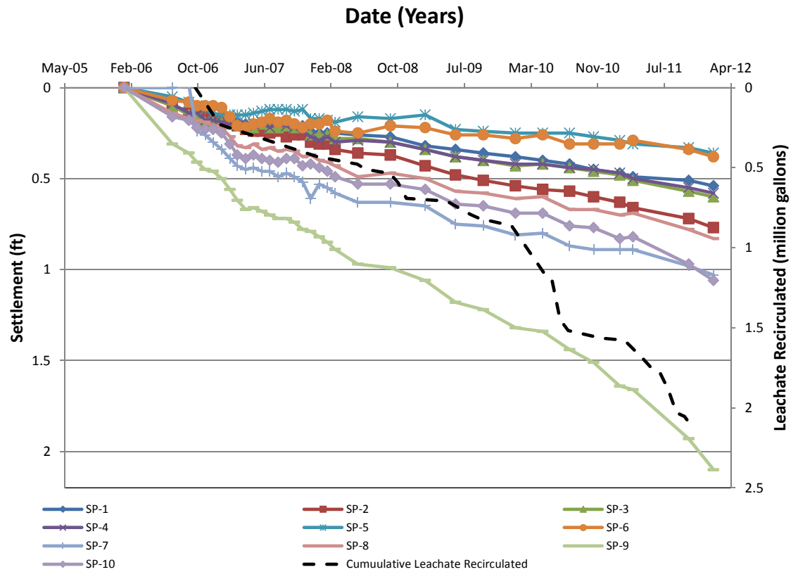
Figure 4-16 – Cumulative Settlement
