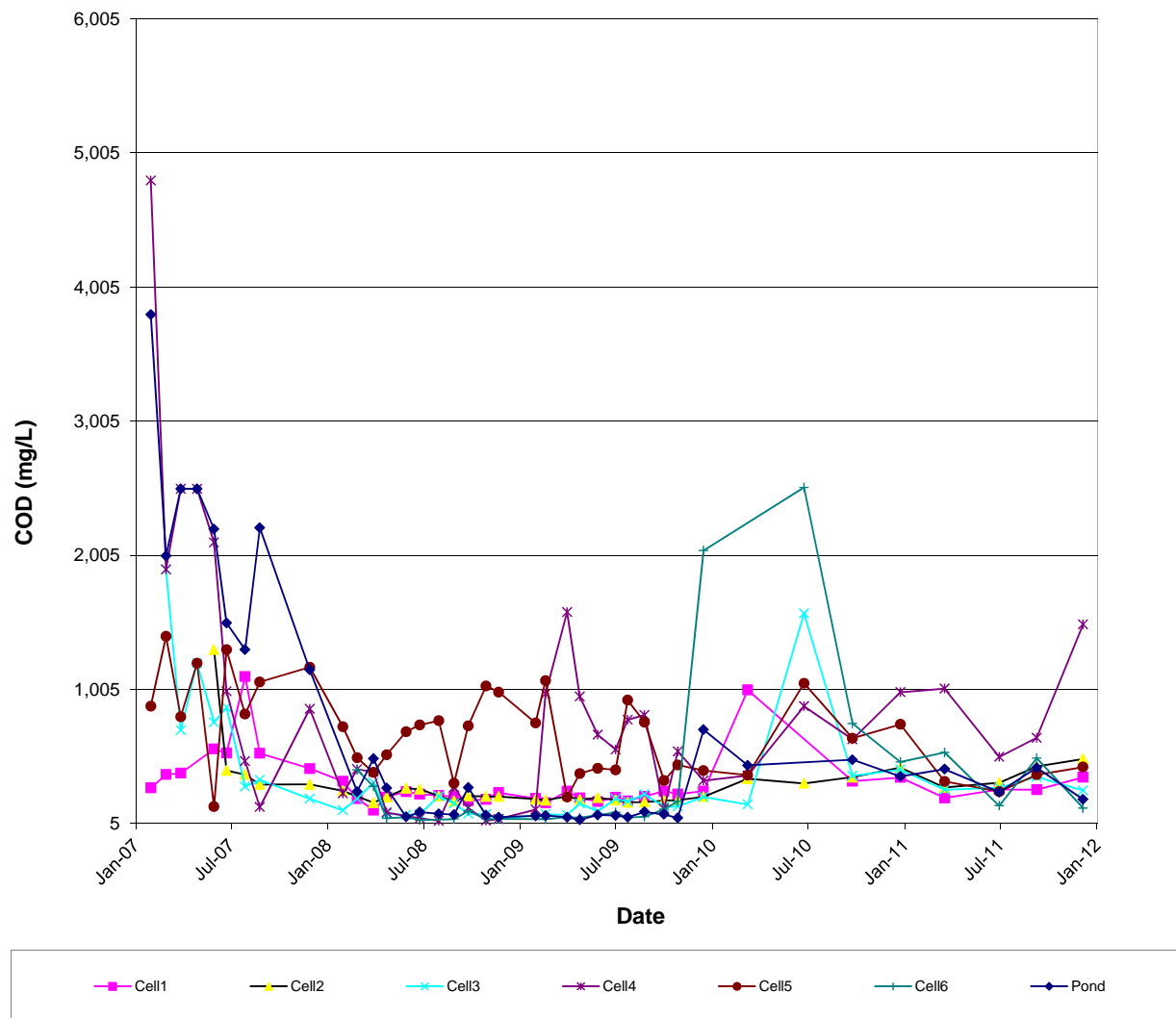
Figure 4-9 – COD of Leachate from Cells 1-6 and Pond in LCS
