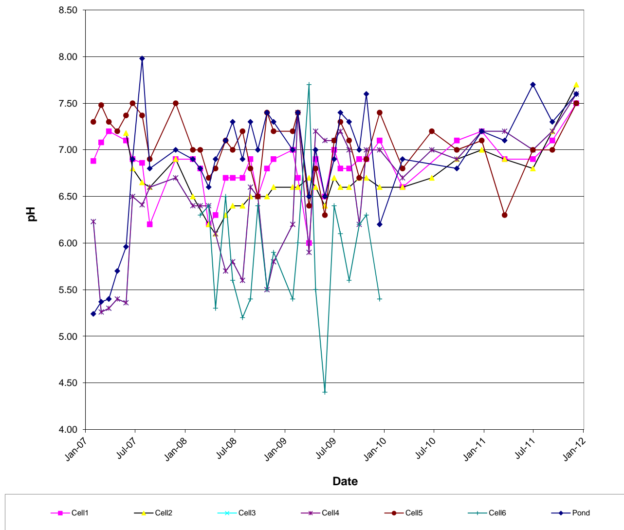
Figure 4-11 – pH of Leachate from Cells 1-6 and Pond in LCS
