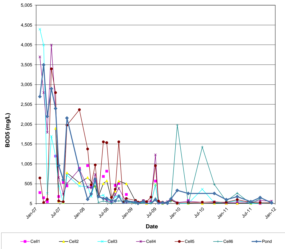
Figure 4-7 – BOD 5 of Leachate from Cells 1-6 and Pond in LCS
