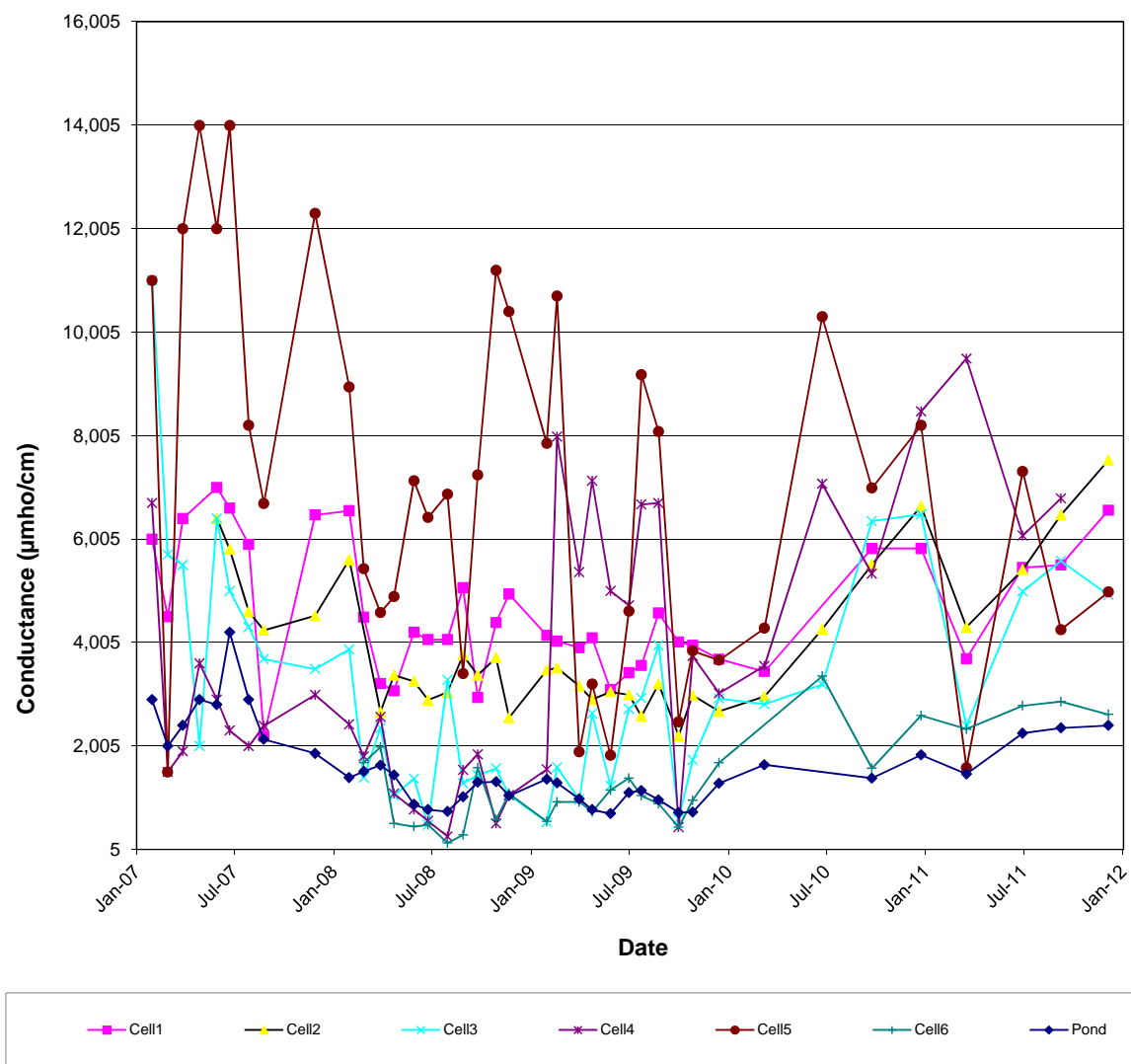
Figure 4-8 – Specific Conductance of Leachate from Cells 1-6 and Pond in LCS
