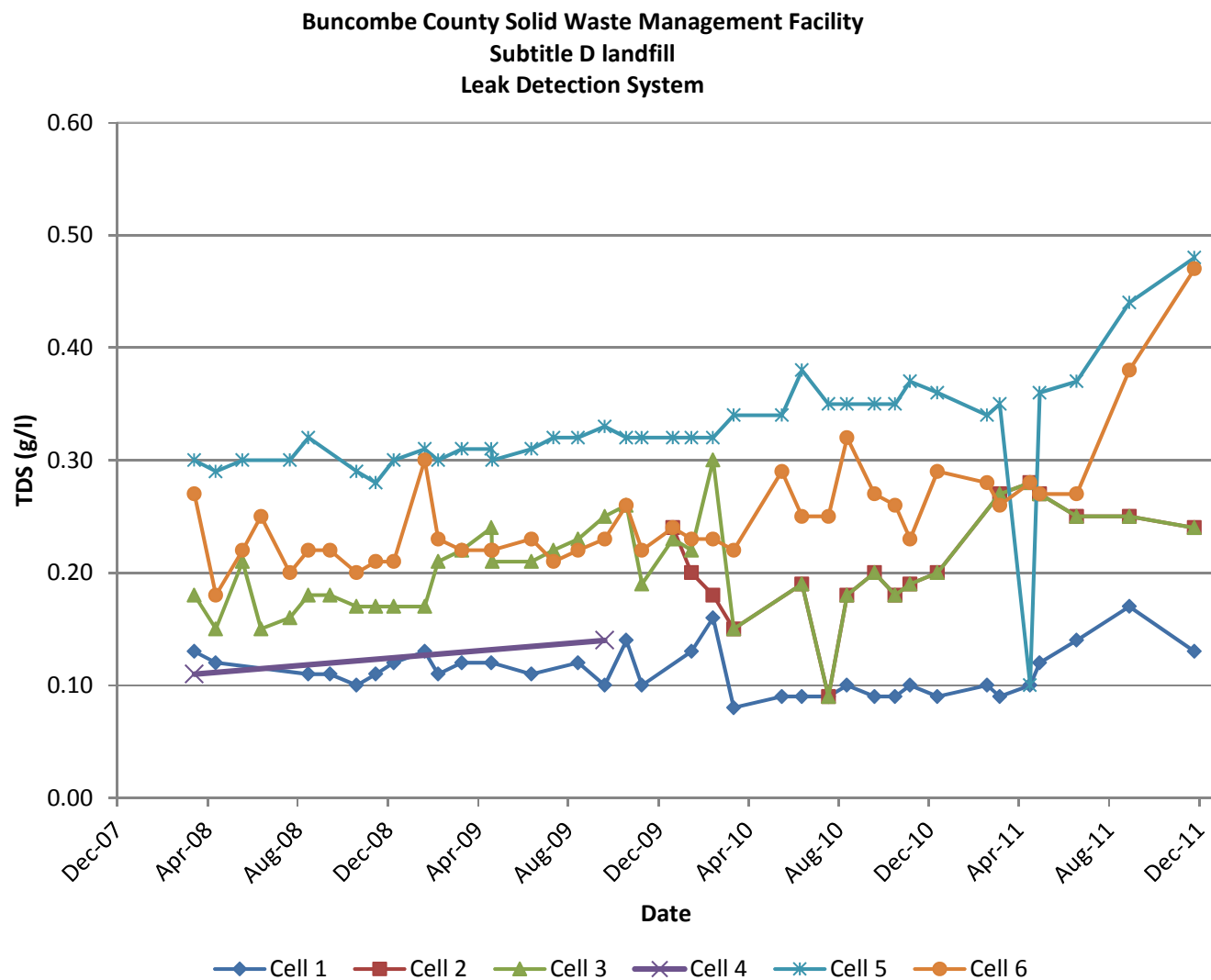
Figure 4-4 – Total Dissolved Solids of Liquids for Cells 1-6 in Leak Detection Zone
