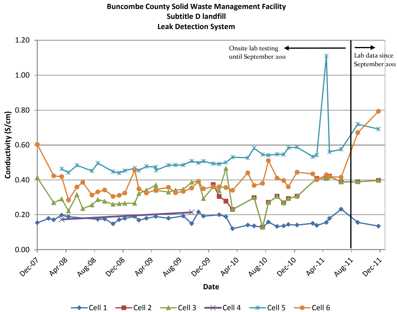
Figure 4-5 – Specific Conductance of Liquids for Cells 1-6 in Leak Detection Zone
