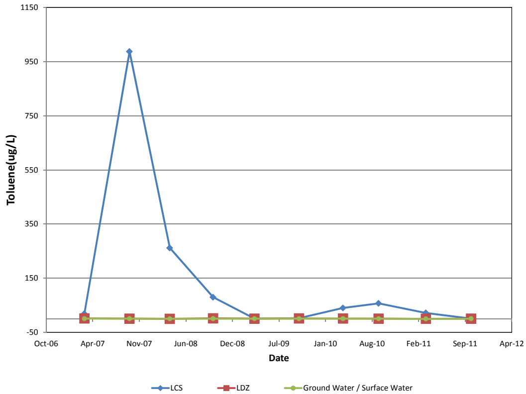
Figure 5-3 – Toluene of LCS, LDZ and GW/SW Samples (Values are averages of testing results for the six cells and all GW/SW monitoring wells)
