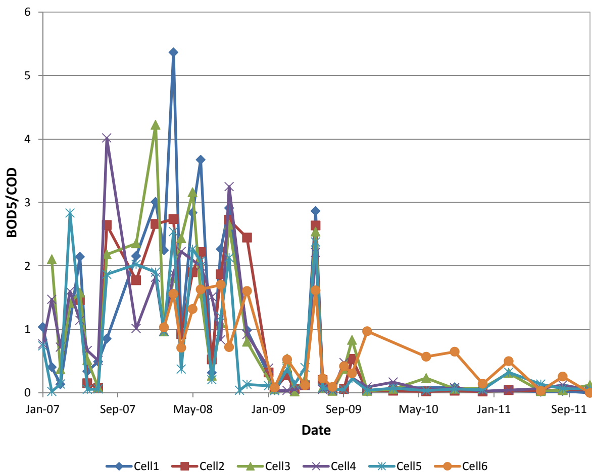
Figure 5-7 – BOD 5 /COD Ratio of LCS in Cells 1-6
