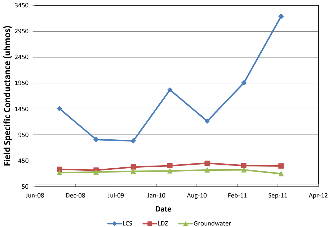
Figure 5-2 – Conductance of LCS, LDZ, and GW Samples (Values are averages of testing results for the six cells and all GW monitoring wells)
