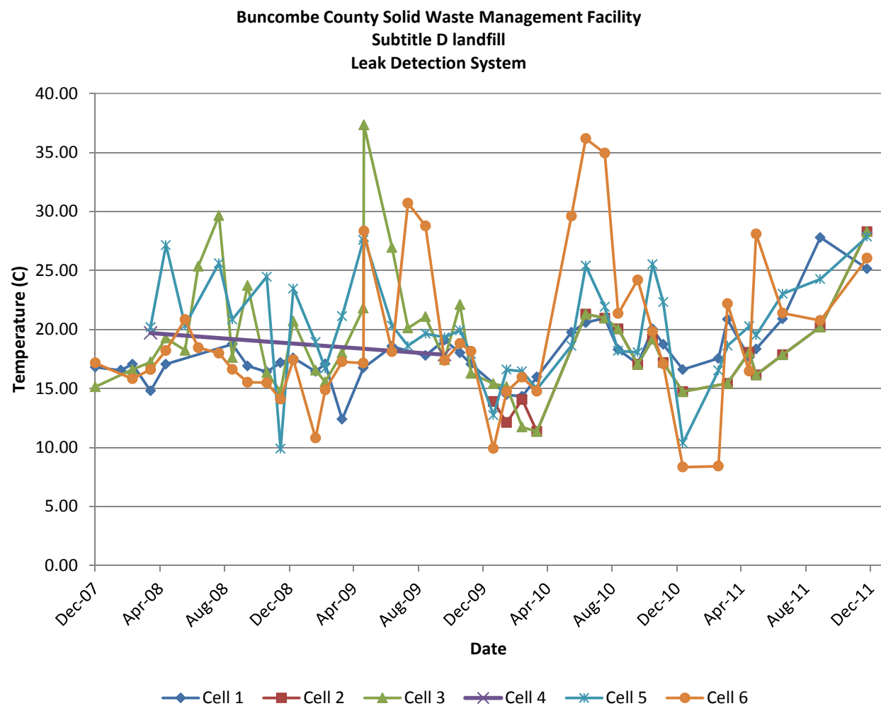
Figure 4-3 – Temperature of Liquids for Cells 1-6 in Leak Detection Zone
