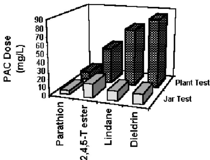
Figure 3.1. PAC Doses Required to Remove 99% of the Pesticide from Jar and Plant Tests. Initial concentration of each pesticide is 10 \mu\text{g/L} (Data from Najm et al, 1991).
