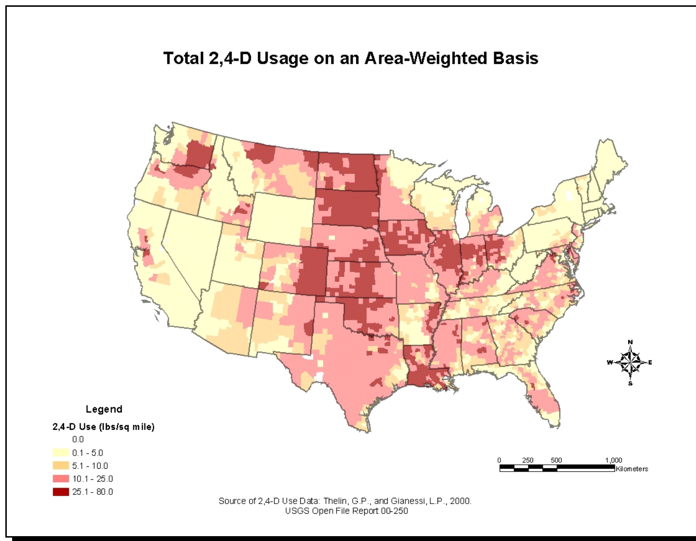
Figure 1. Estimated 2,4-D usage (lbs ae/square mile). The estimates are based on pesticide use rates compiled by the National Center for Food and Agricultural Policy (NCFAP) and modified by Thelin, G.P. and Gianessi, L.P., 2000 (USGS Open-File Report 00-250)
