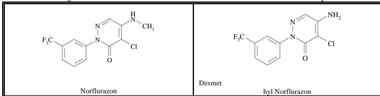
Figure B. Chemical names and structures of norflurazon and its metabolite in plants.
