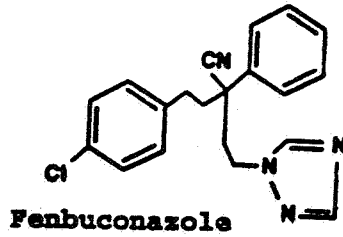
Figure 1. Structures of Related Triazole Pesticides. 010669
