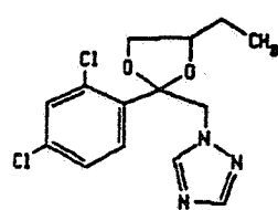
Propiconazole
