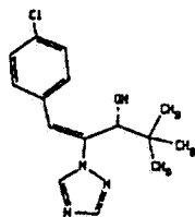
Uniconazole
