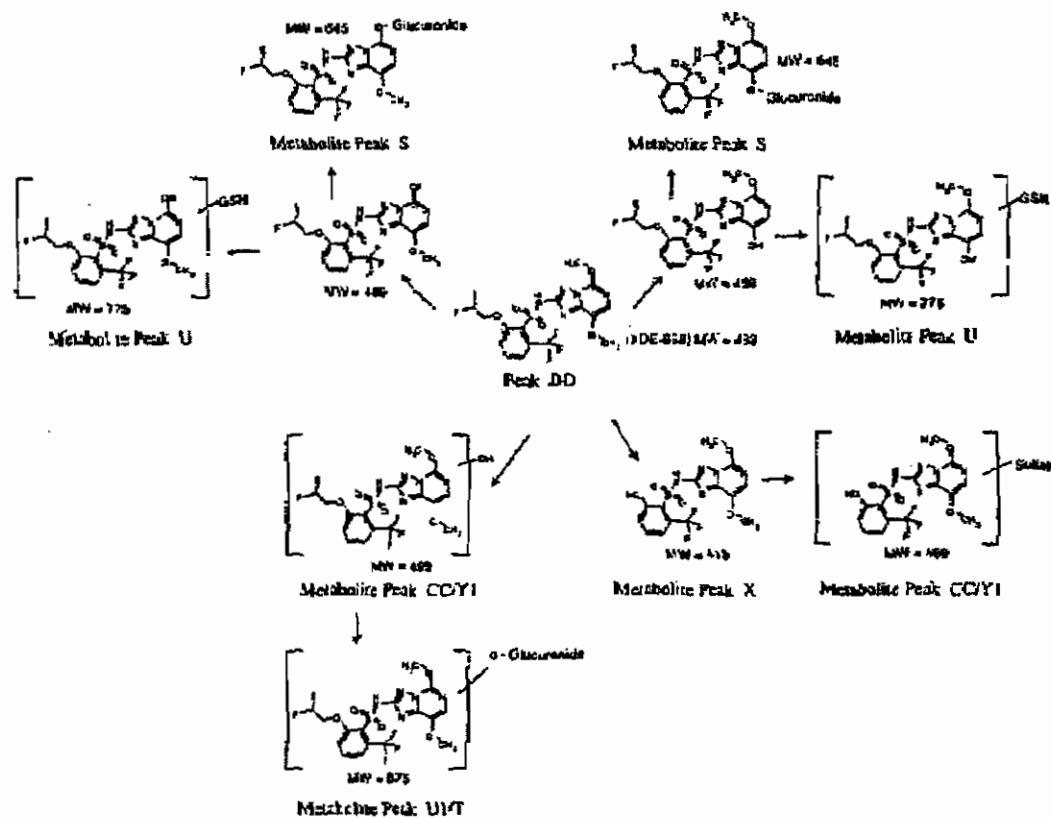
Figure 1. Proposed metabolism pathway for XDE-638 (Penoxsulam) in the rat. Taken from Figure 16, p. 78, MRID 45830927.
