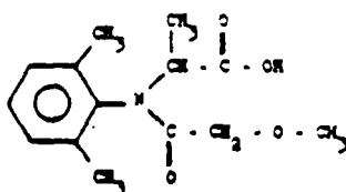
CGA 68936, N-(2,6-dimethylphenyl)-N-(2'-methoxyacetyl)-alanine
