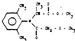
CGA 48988, N-(2,6-dimethylphenyl)-N-(2'-methoxyacetyl)-alanine methyl ester
