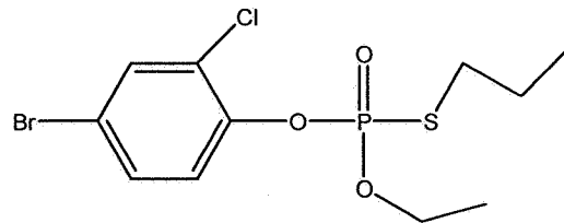
Profenophos
