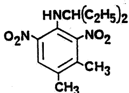
N-(1-ETHYLPROPYL)-3,4-DIMETHYL-2,6-DINITRO- BENZENAMINE
