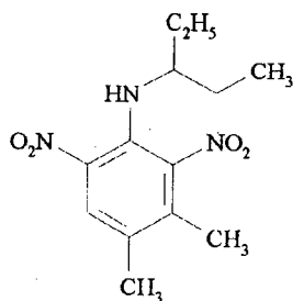
Pendimethalin
