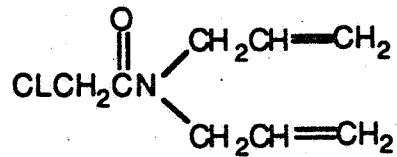
Allidochlor
