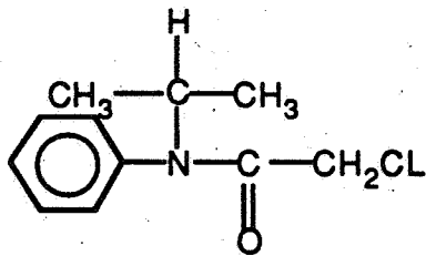
Propachlor
