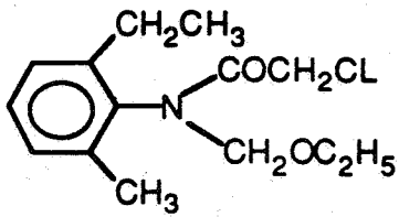
Acetochlor
