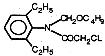
Butachlor
