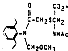
Tertiary Mercapturate (5)
