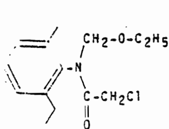
Acetochlor
