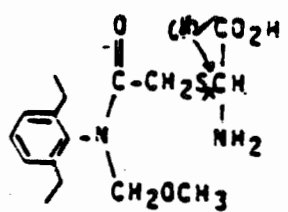
Tertiary Mercapturate (5)
