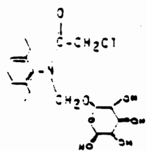
Glucuronide Conjugate (3)
