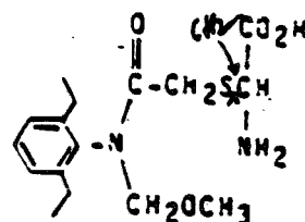
Tertiary Mercapturate (5)
