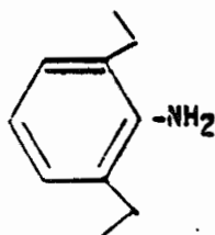
DEA
