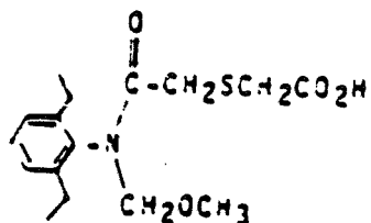
Secondary Mercapturate (4)
