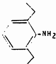
DEA
