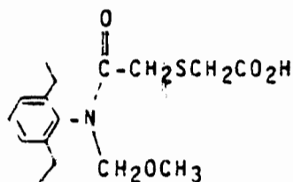
Secondary Mercapturate (4)
