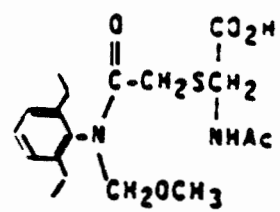
Tertiary Mercapturate (5)
