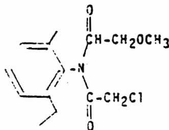
Metalochlor
