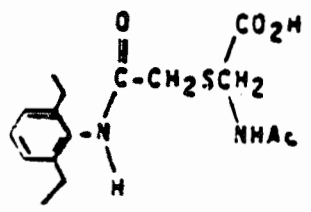
Secondary Mercapturate (4)
