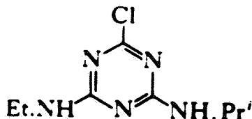
Atrazine
