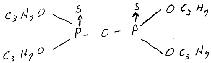
O,O,O,O-Tetra-n-propyl dithiopyro phosphate - Aspon
