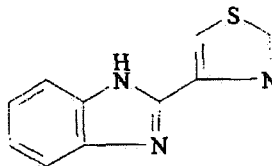
Figure 1. Thiabendazole
