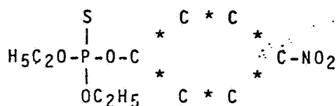
Ethylparathion
