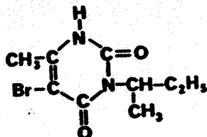
5-Bromo-3-sec-butyl-6-methyluracil
