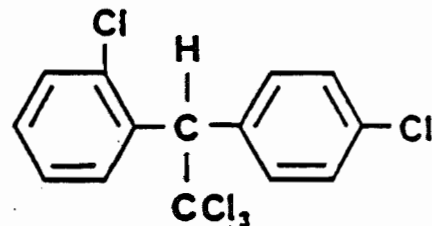
1-(2-Chlorophenyl)-1-(4'-chloro- phenyl)-2,2,2-trichloroethane
