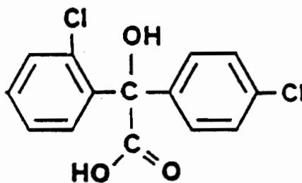
2,4'-Dichlorobenzilic acid
