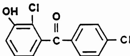
3-Hydroxy-2,4'-dichlorobenzophenone
