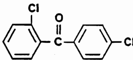
2,4'-Dichlorobenzophenone
