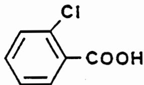
2-Chlorobenzoic acid
