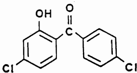
2-Hydroxy-4,4'-dichlorobenzophenone
