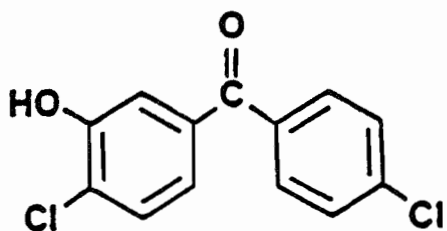
3-Hydroxy-4,4'-dichlorobenzophenone
