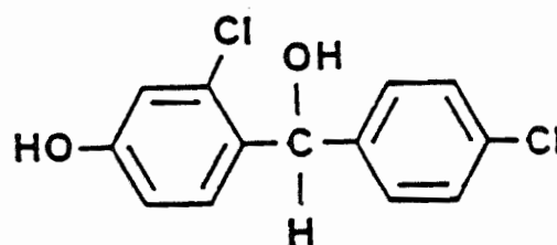
4-Hydroxy-2,4'-dichlorobenzhydrol
