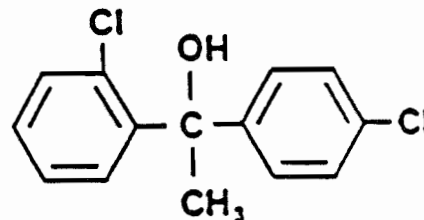
1-(2-Chlorophenyl)-1(4'- chlorophenyl)-ethanol
