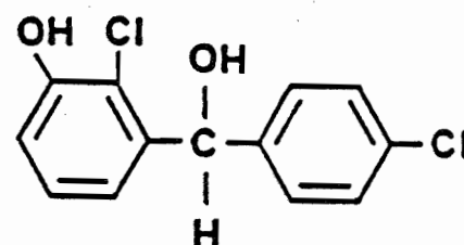
3-Hydroxy-2,4'-dichlorobenzhydrol
