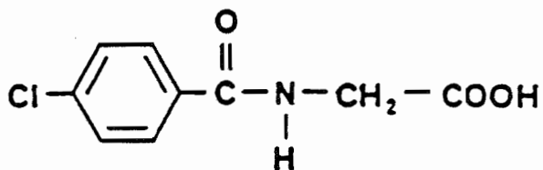
4-Chlorhippuric acid
