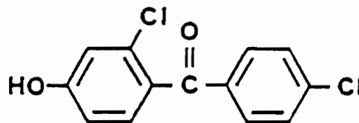
4-Hydroxy-2,4'-dichlorobenzophenone
