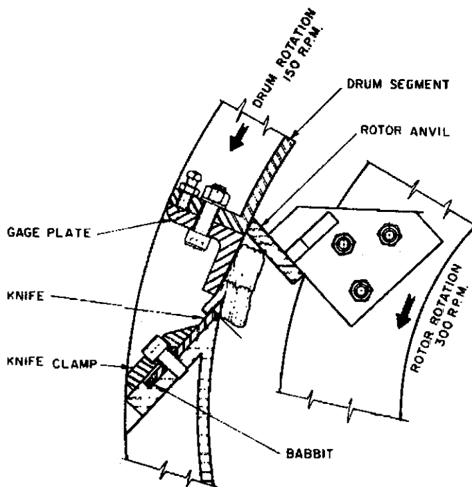
Figure 3-2. Chip thickness slicer showing oversize chip being split.
