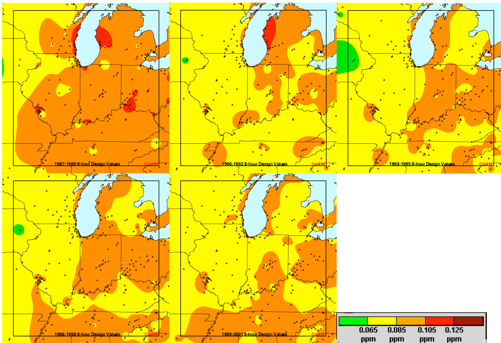
Figure 2. 8-Hour Design Values for 1987-1989, 1990-1992, 1993-1995, 1996-1998, and 1999-2001
