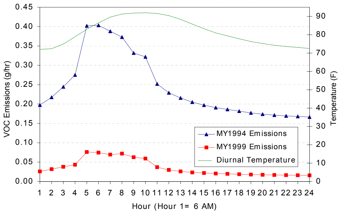
LDGV CY2005 Hourly Diurnal and Resting Loss Emissions
