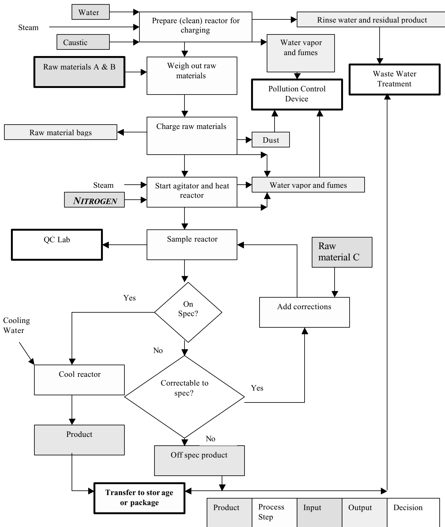
Example 5-3: Flow Diagram for a Pressurized Reactor Operation
