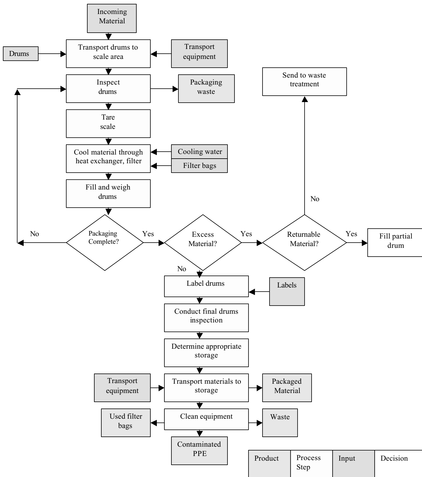
Example 5-4: Flow Diagram for Packaging Area
