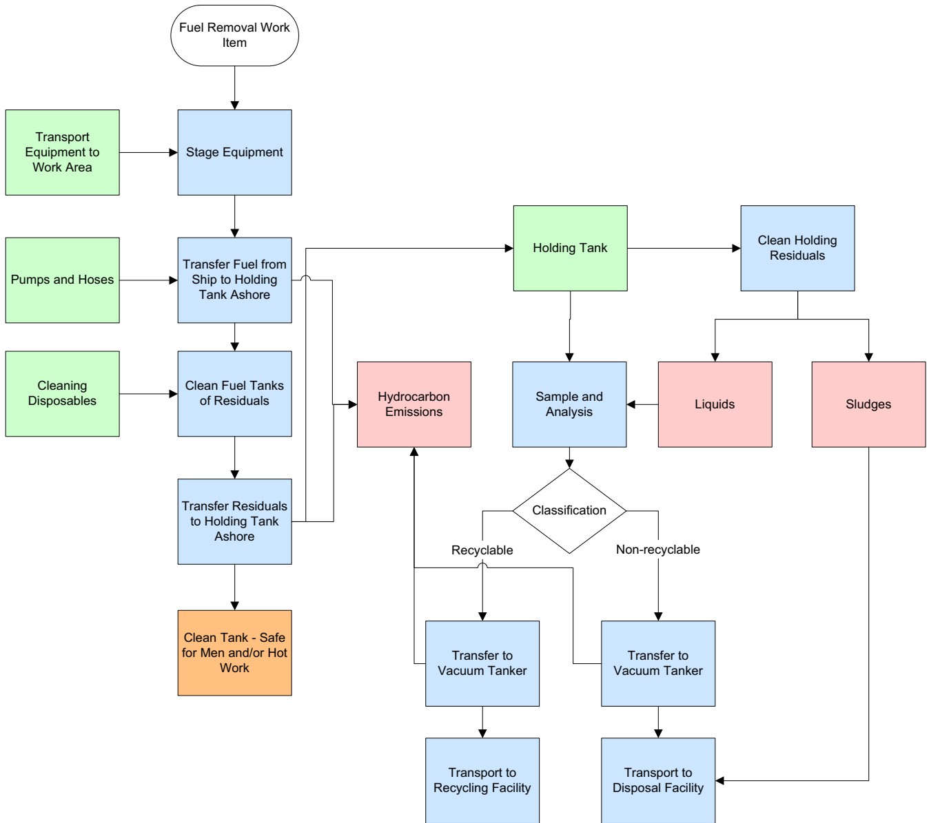
Example 5-11: Flow Diagram and Aspects Form for Ship's Fuel Removal
