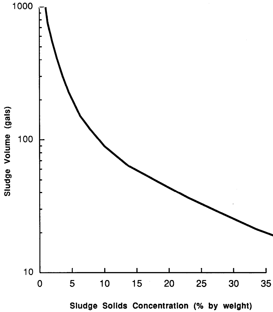
Figure A-2 - Sludge Volume Vs Sludge Solids Concentration
