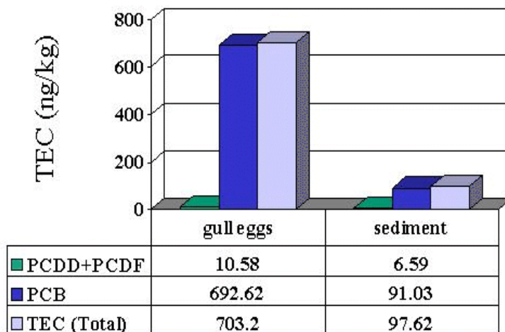
Figure 8. Bird TECs calculated for eggs versus sediment.
