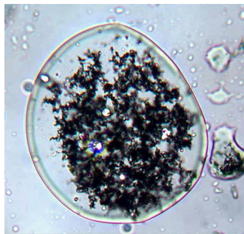
Figure 13. Nanoscale zero-valent iron encapsulated in an emulsion droplet. These nanoparticles have been used for remediation of sites contaminated with various organic pollutants. (Image courtesy of Dr. Jacqueline W. Quinn, Kennedy Space Center, NASA)
