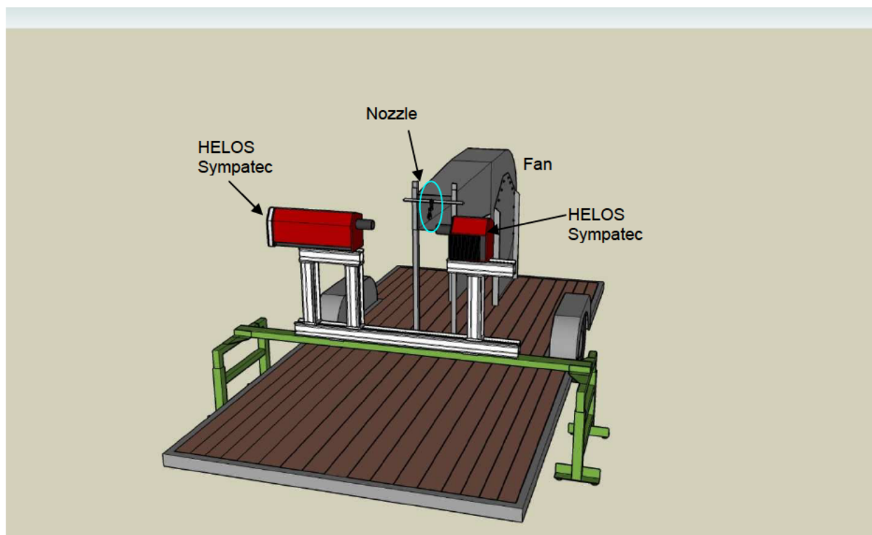
Figure 4. Overview of HSWT with enclosure removed for clarity.
