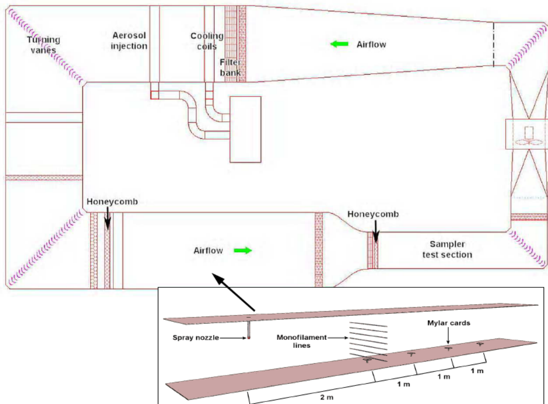
Figure 2. EPA's aerosol wind tunnel (AWT).
