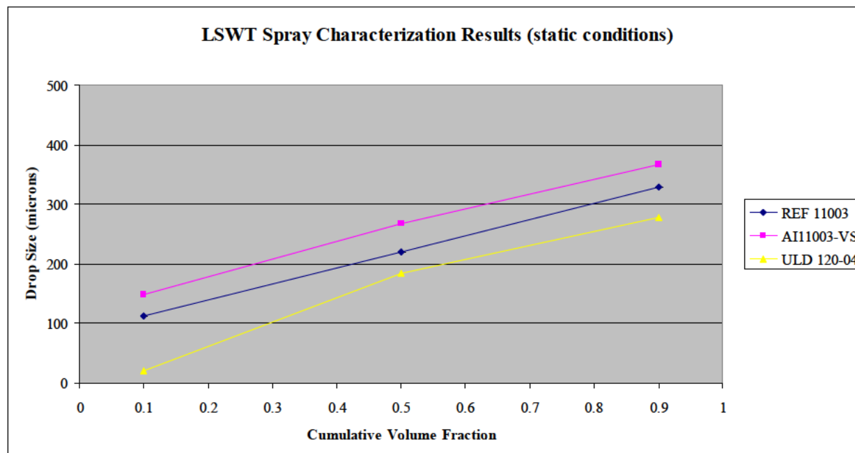
Figure 6. LSWT spray characterization results under static wind conditions.
