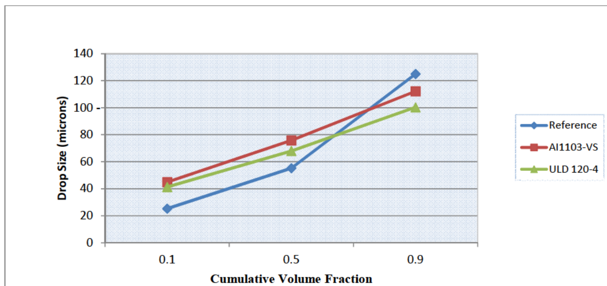
Figure 7. Example of LSWT spray characterization at the 2-meter flux plane and 20 cm height.
