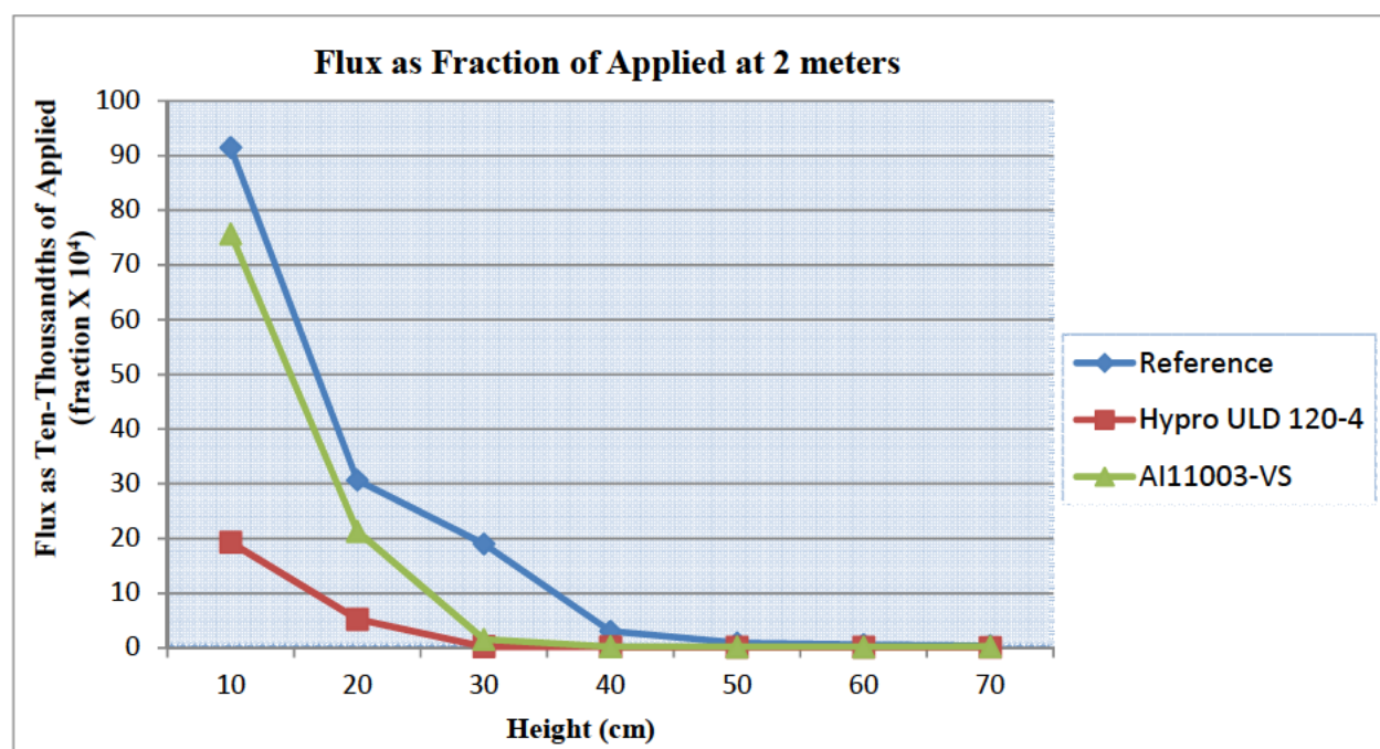
Figure 8. LSWT spray flux 2 meters from the nozzle (flux vs. height for three nozzles).
