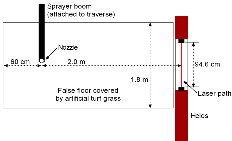
Figure 5. Schematic diagram of the set up for droplet sizing measurements 2 m downwind.
