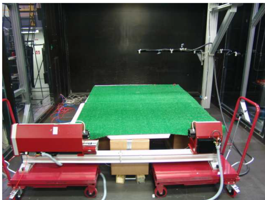
Figure 3. AWT setup for low-speed DRT tests.
