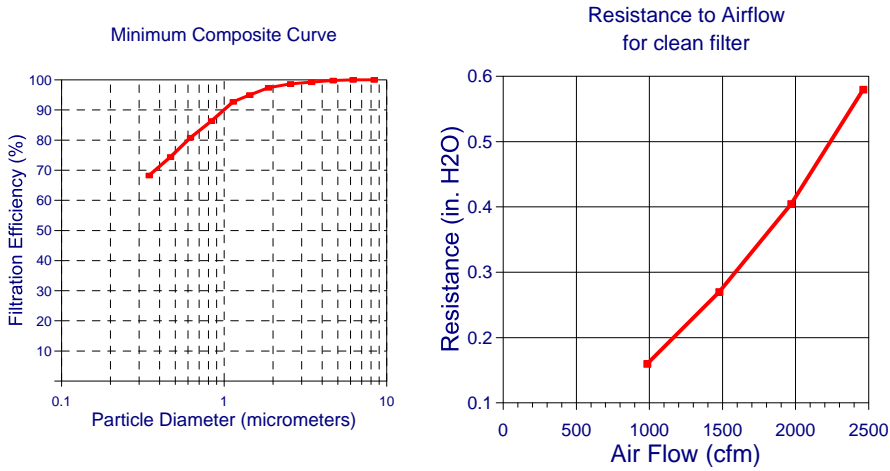
Figure A-1. Filtration Efficiency and Flow Resistance Curves for Aeolus Synthetic Minipleat V-cell SMV-M14-2424 Filter.
