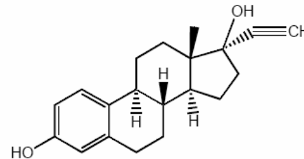
Ethinyl-Estradiol
