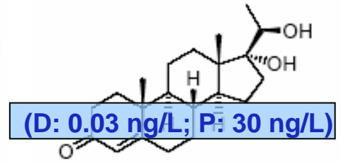
17α-20B-Dihydroxyprogesterone
