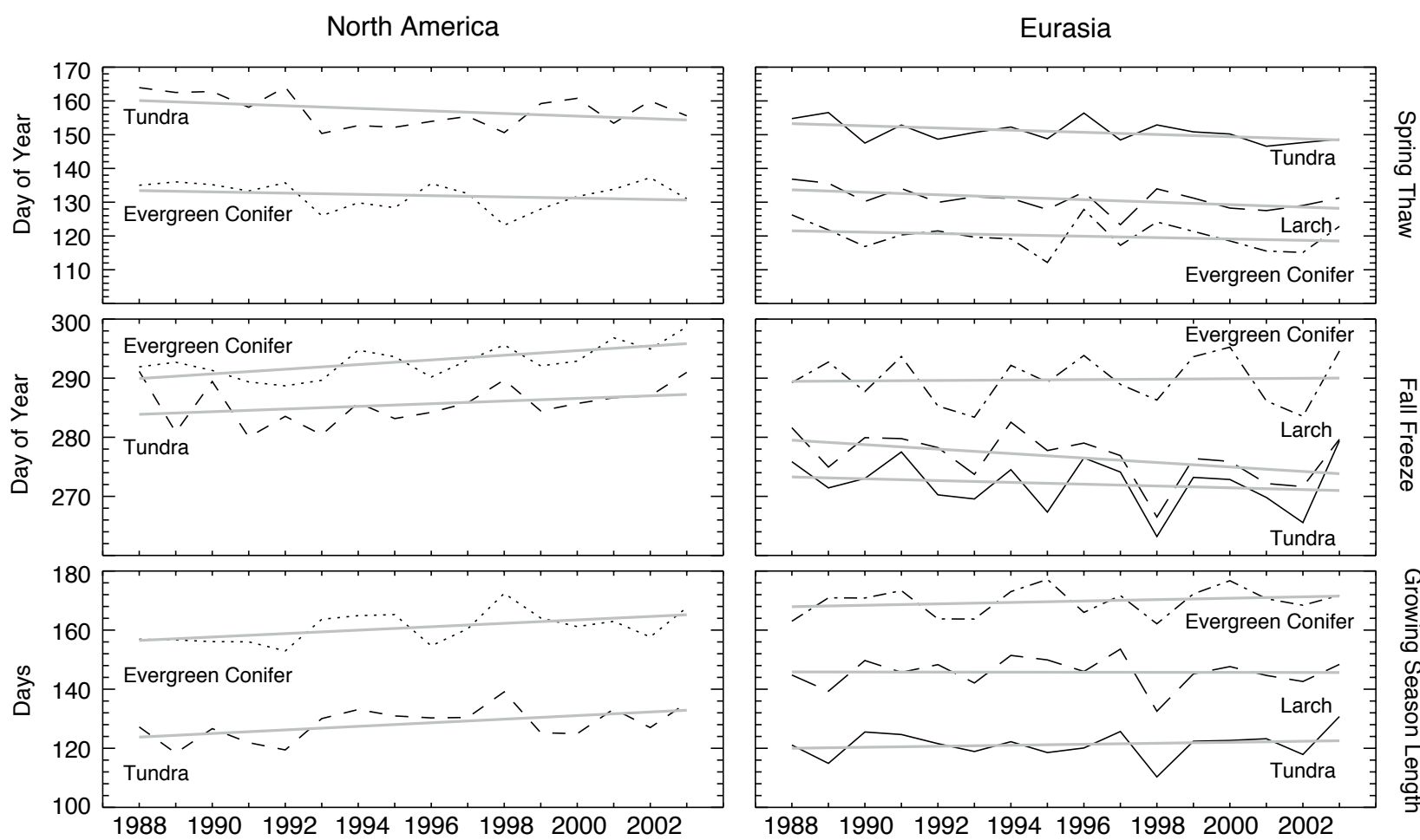
Figure 3. Biome level trends in thaw, freeze and growing season length for North America and Eurasia. Smith et al. in press.
