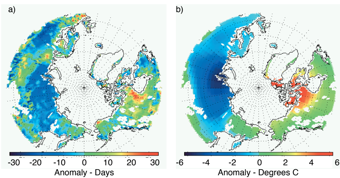
Figure 4. 1998 anomaly in fall freeze (a) and fall surface air temperature (b). Air temperature data from Hansen et al. 2001.
