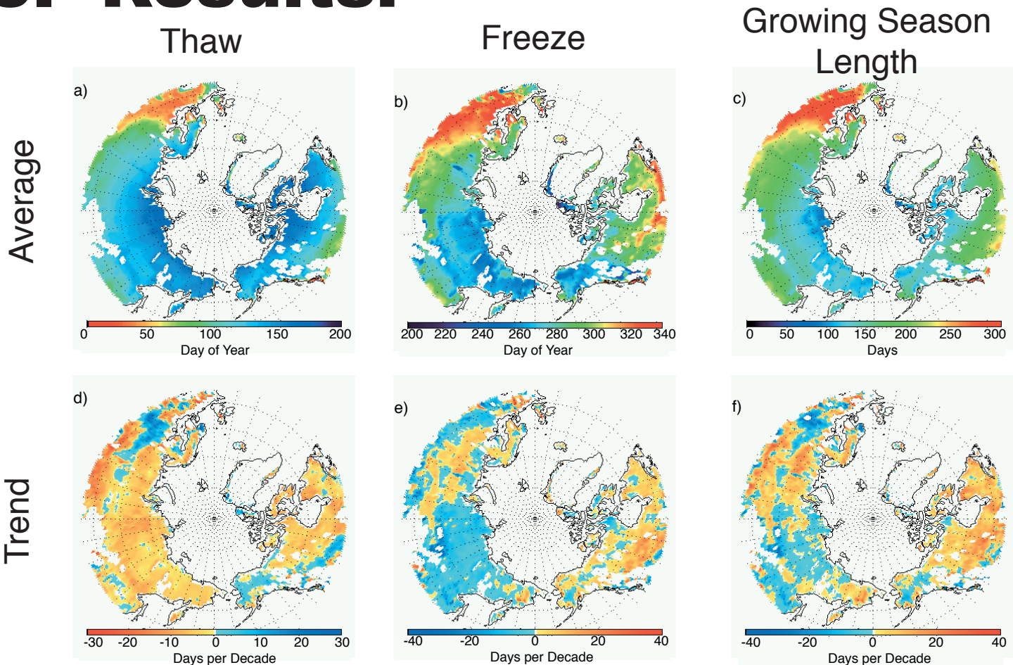
Figure 2. Average date of thaw (a), freeze (b) and growing season length (c) for all latitudes north of 45° N. Trend in thaw (d), freeze (e) and growing season length (f) over the period 1988-2002. Smith et al. in press.
