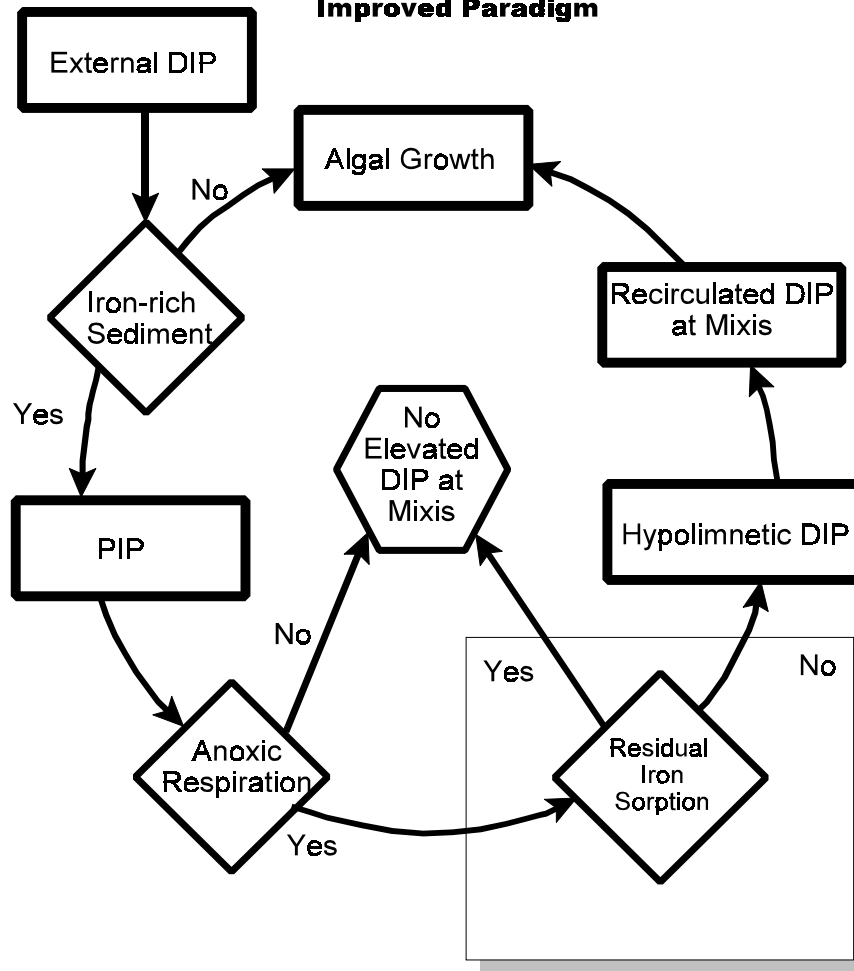
Figure 1. The phosphorus cycling program in lakes is based on data from systems in northern temperate regions. Phosphorus sorbs to iron-rich sediments from tributaries and runoff to form particulate inorganic phosphorus (PIP). Anoxic respiration in the hypolimnion of north-temperate lakes creates strongly reducing conditions that liberate dissolved inorganic phosphorus (DIP) from settling particulates. Hypolimnetic DIP steadily increases during summer stratification as phosphorus is liberated, and is mixed throughout the water column at fall overturn. This paradigm fails to explain phosphorus cycling in Southeastern Piedmont lakes. No increase in DIP is found in the anoxic hypolimnion during summer stratification, nor is an increase in DIP observed during fall overturn in Southeastern Piedmont lakes. It is hypothesized that the conventional paradigm is not appropriate in iron-rich Southeastern Piedmont systems because: (1) iron-oxide sorption reduces the bioavailability of DIP, and (2) the abundance of oxidized iron prevents DIP accumulation in the anoxic hypolimnion.
