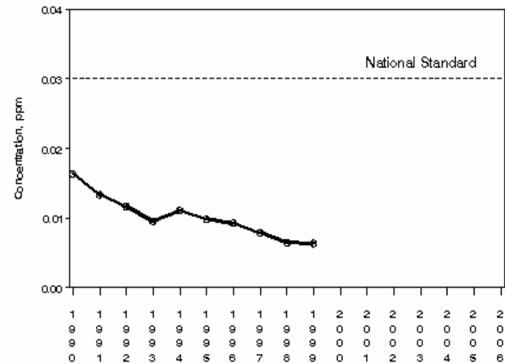
SO 2 Air Quality, 1990 — 2006 (Based on Annual Arithmetic Average) New York, NY SITE= 360470011 POC= 1
