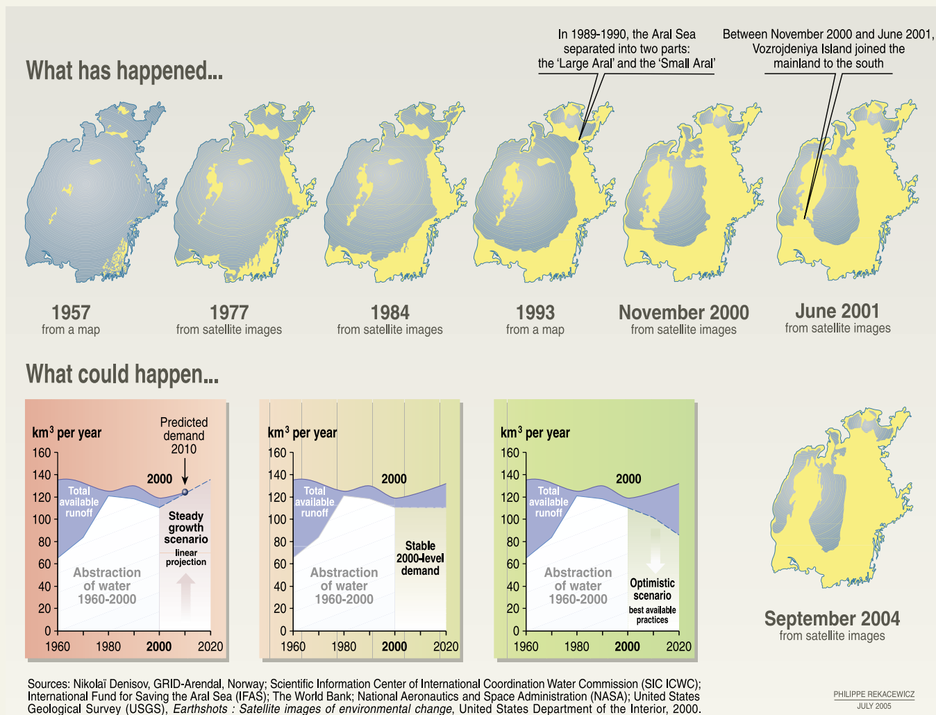
Figure 4.2. DECLINE IN SIZE OF THE ARAL SEA SINCE 1957 (C20.4.1)
