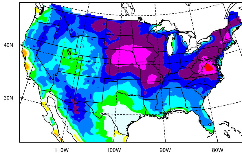
HGR-HAD JJA TA Future (2100) A2 Change
