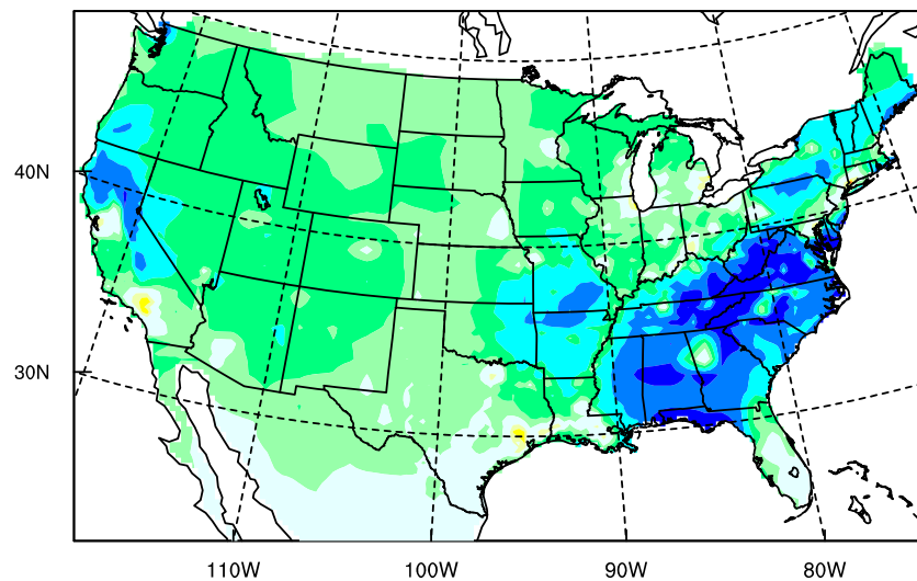
AQM/PGR JJA Ozone Future (2100) B1 Change
