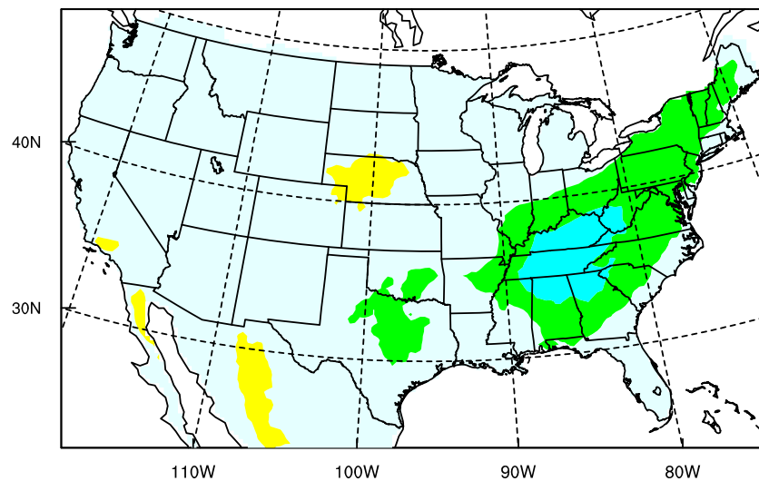
PGR-PCM JJA TA Future (2100) B1 Change
