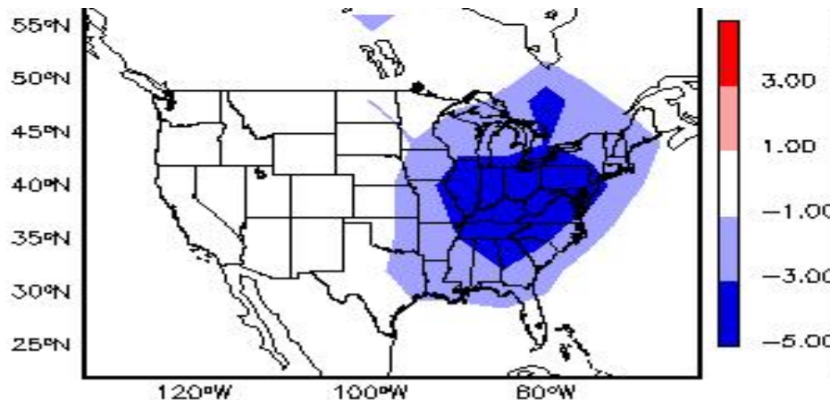
\Delta(2050 \text{ emissions \& } 2000 \text{ climate})
