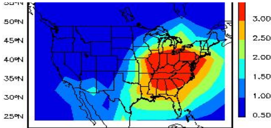
2000 conditions: sulfate, \mu\text{g m}^{-3}
