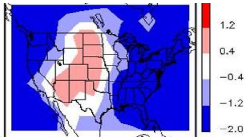
\Delta (2000 emissions & 2050 climate)
