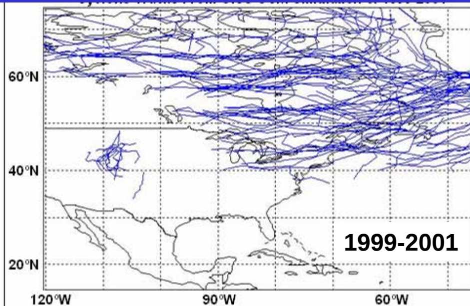
2000 climate
