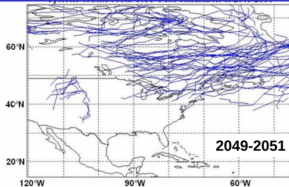
2050 climate
