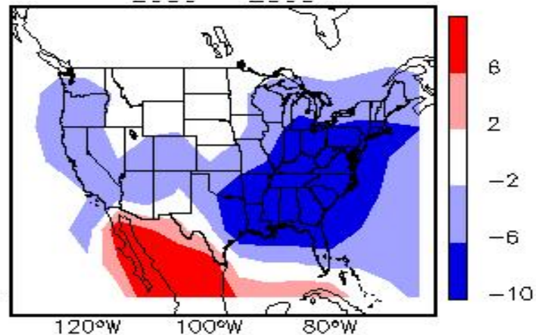
\Delta (2050 emissions & climate)
