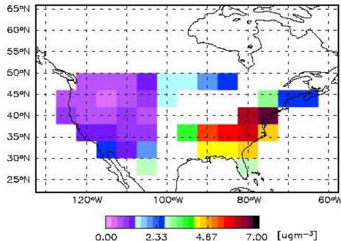
IMPROVE
