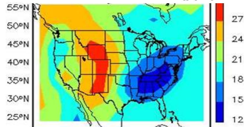
1999-2001 PRB ozone (ppb)
