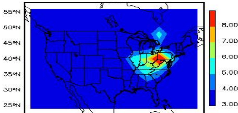
\Delta(2050 \text{ emissions \& } 2000 \text{ climate})
