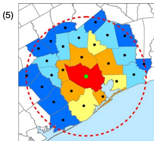
(5) Spatially distributed emissions values based on the spatial weighting scheme. Note that red indicates areas of high emissions influence and blue represents areas of low influence. Also note that emissions are higher in the center of the buffer zone because as the distance from the county centroid increases the pollutant emissions value decreases as a function of the pollutant buffer distance (listed in Table 5 by pollutant).
