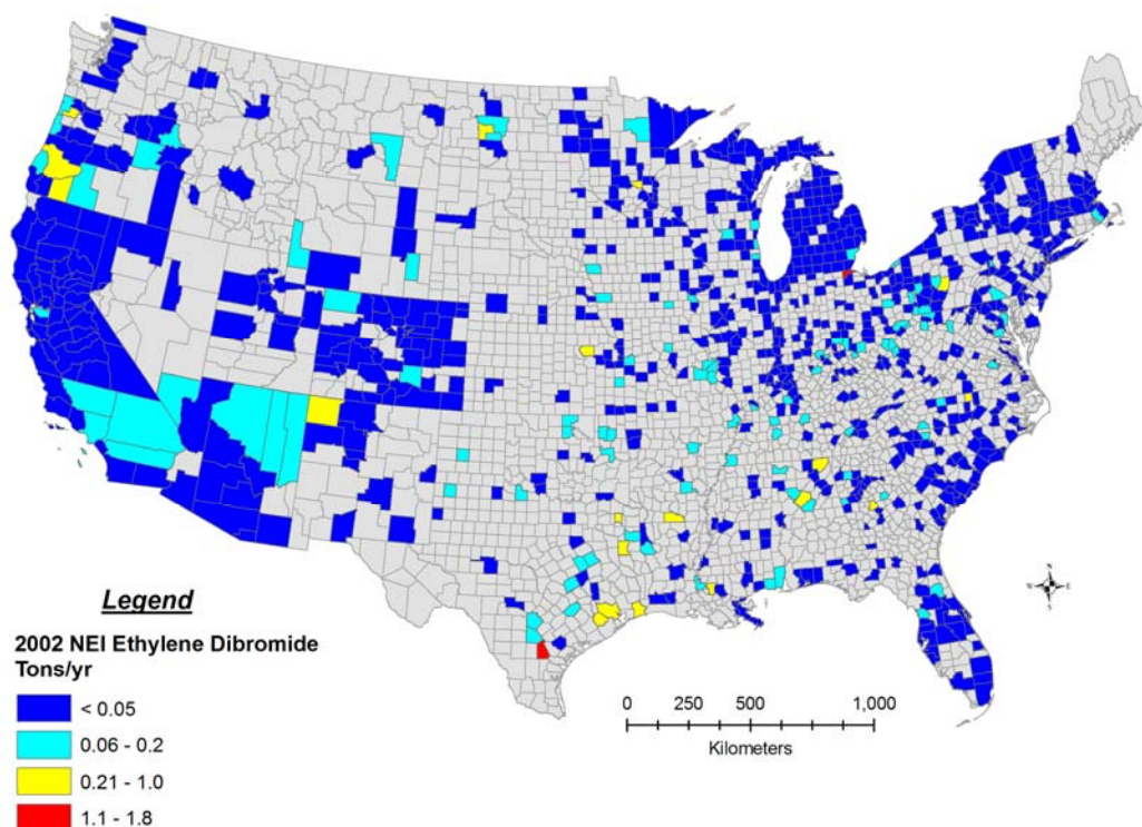
Figure 2-4. Countywide ethylene dibromide emissions (tons/year) as reported in the 2002 NEI. Each county is colored according to the magnitude of its total emissions, with gray indicating no reported emissions.
