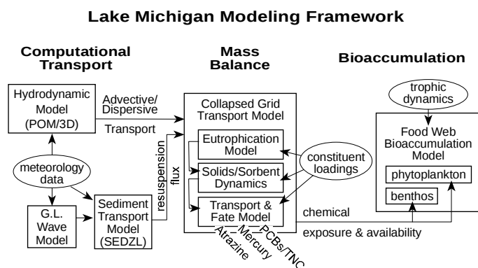
Figure 2. Lake Michigan Modeling Framework.
