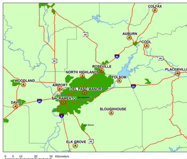
Figure 4. Ground-level ozone monitoring sites in the Sacramento Metropolitan Region.
