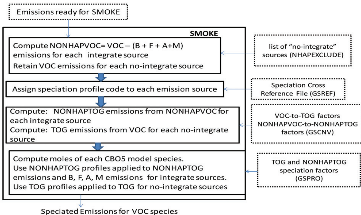
Figure 3-4. Process of integrating BAFM with VOC for use in VOC Speciation
