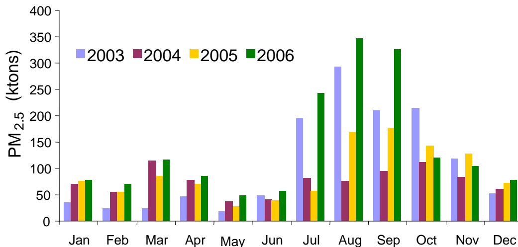
Figure 3-1. Wildfire Emissions in the Contiguous 48 States
