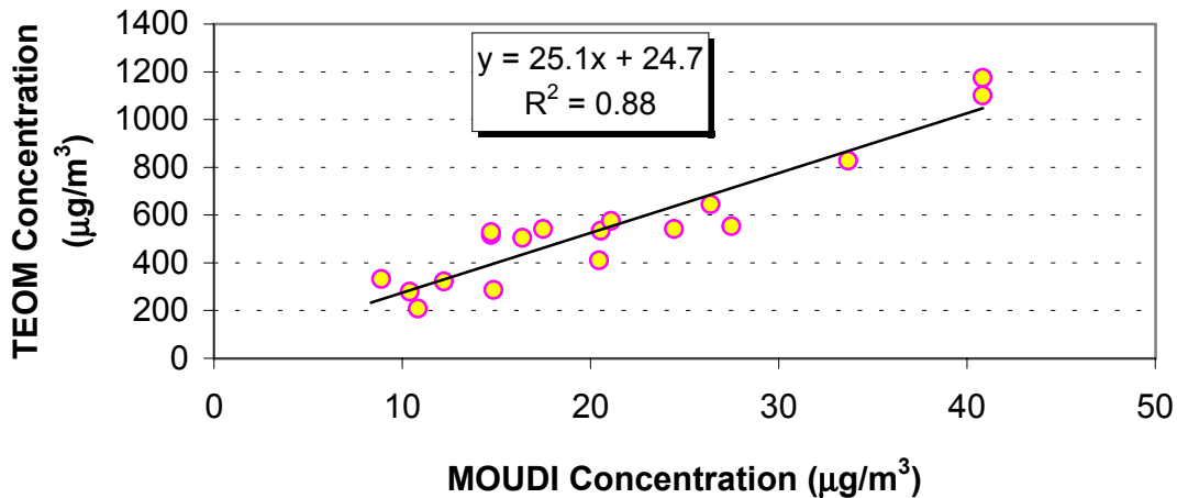
Figure 4. TEOM vs MOUDI Coarse PM Concentrations. TEOM at 50 deg C
