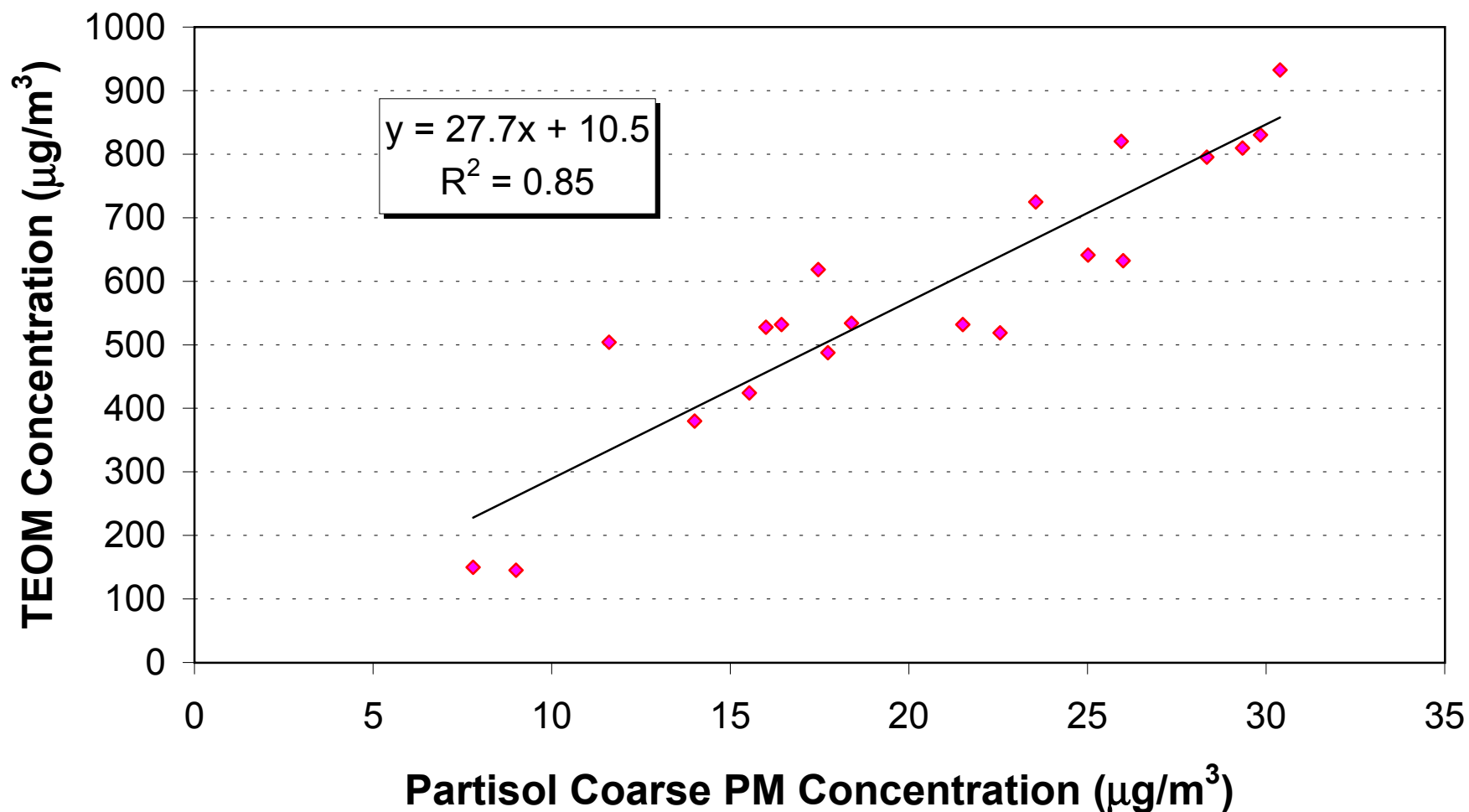
Figure 8. TEOM vs Partisol Coarse PM Concentrations. TEOM at 30 deg C
