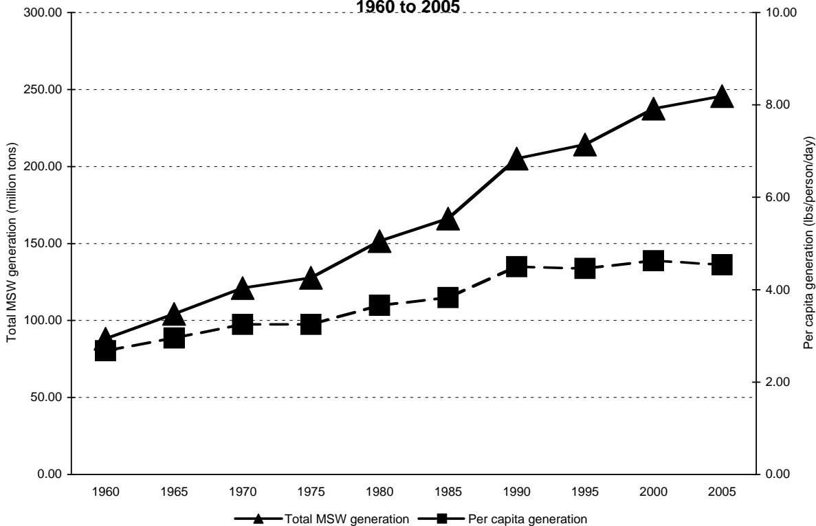
Figure ES-1: MSW Generation Rates, 1960 to 2005
