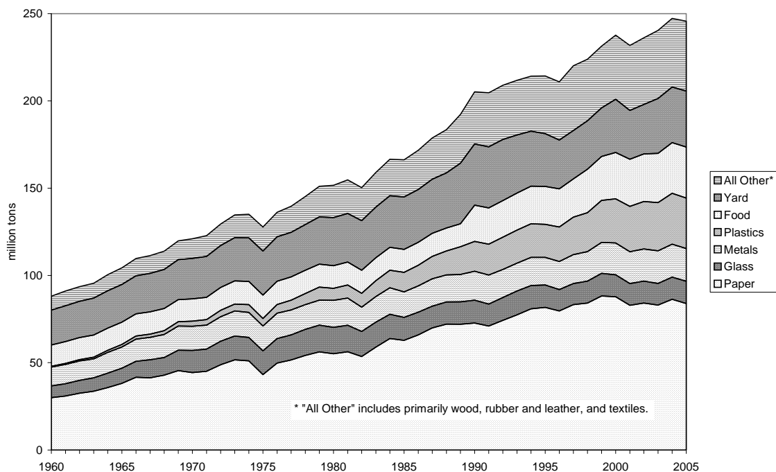
Figure 10. Generation of materials in MSW, 1960 to 2005
