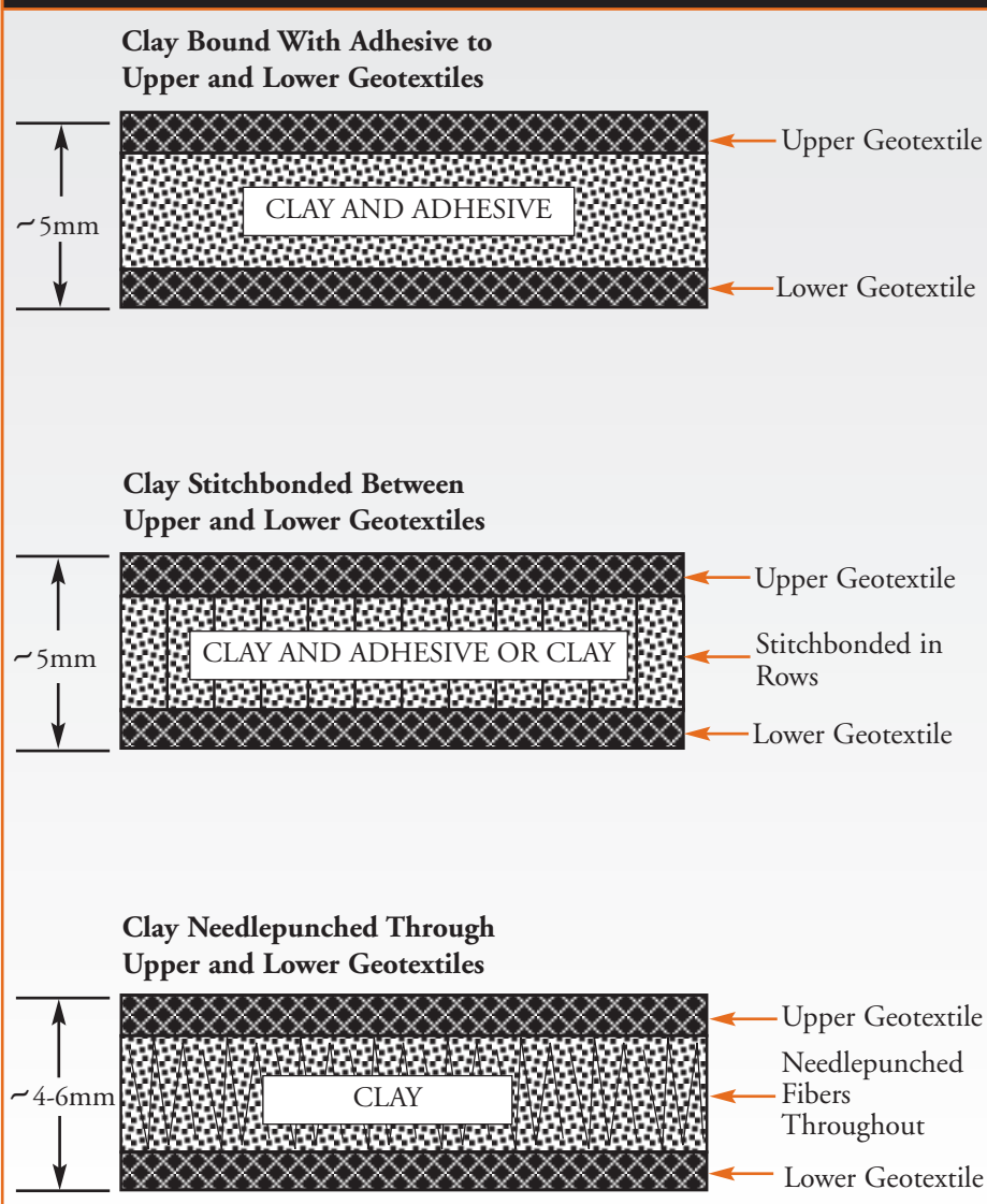
Figure 2. Affixing Bentonite to Geotextiles
