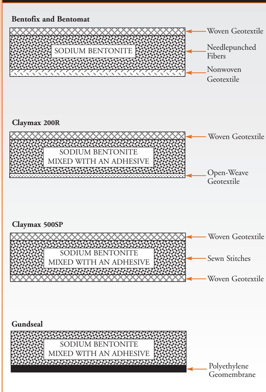
Figure 3. Available GCL Products
