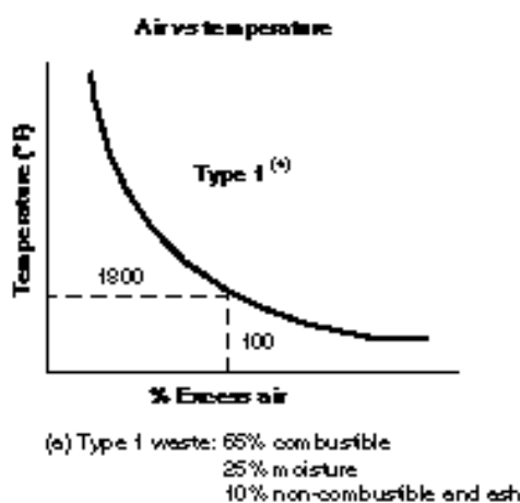
Figure 8-5 Combustion Excess Air Versus Combustion Gas Temperature
