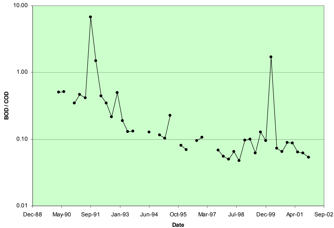
Leachate BOD / COD Ratio
