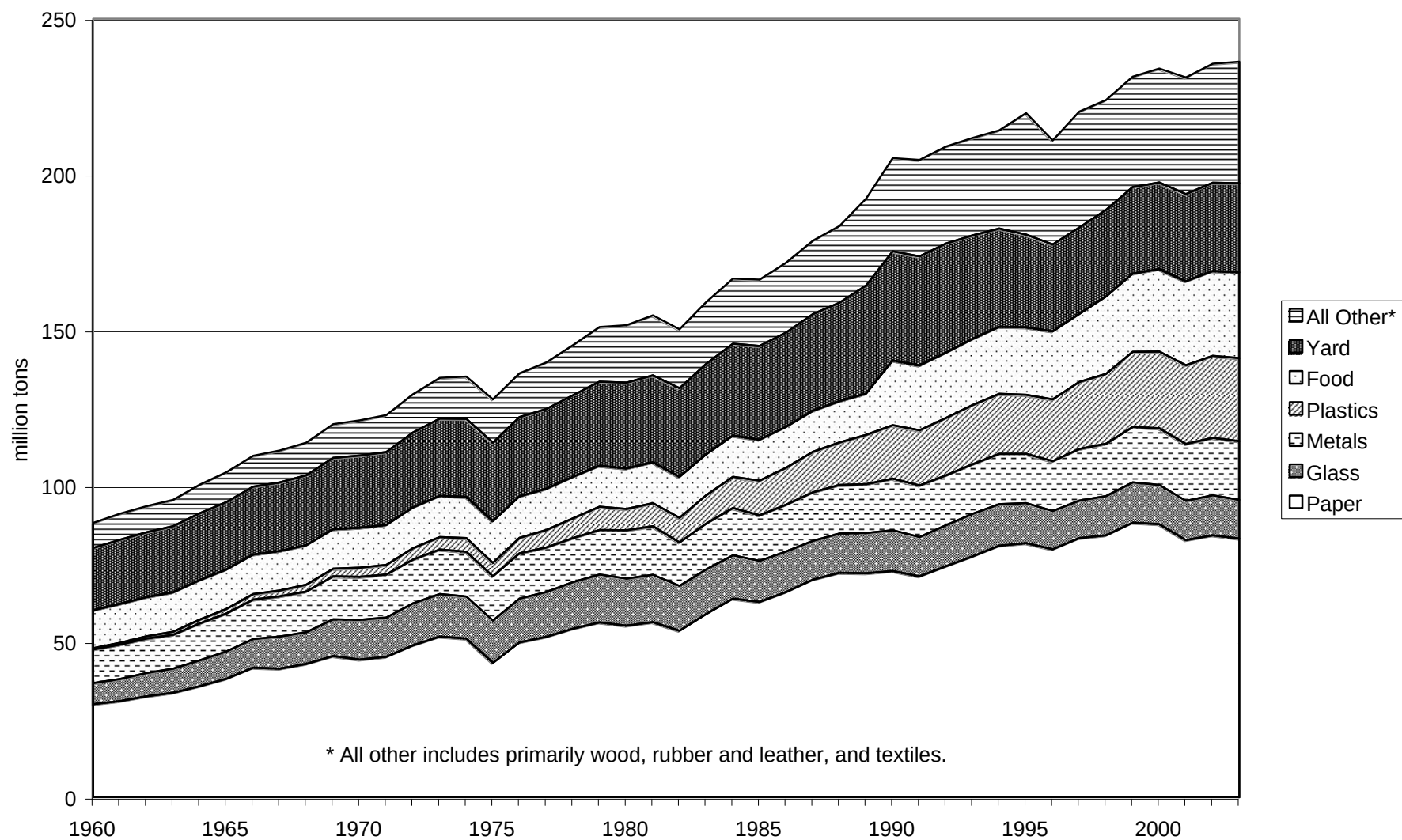
Figure 10. Generation of materials in MSW, 1960 to 2003
