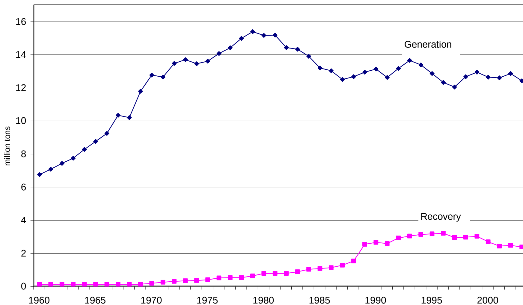
Figure 5. Glass generation and recovery, 1960 to 2003
