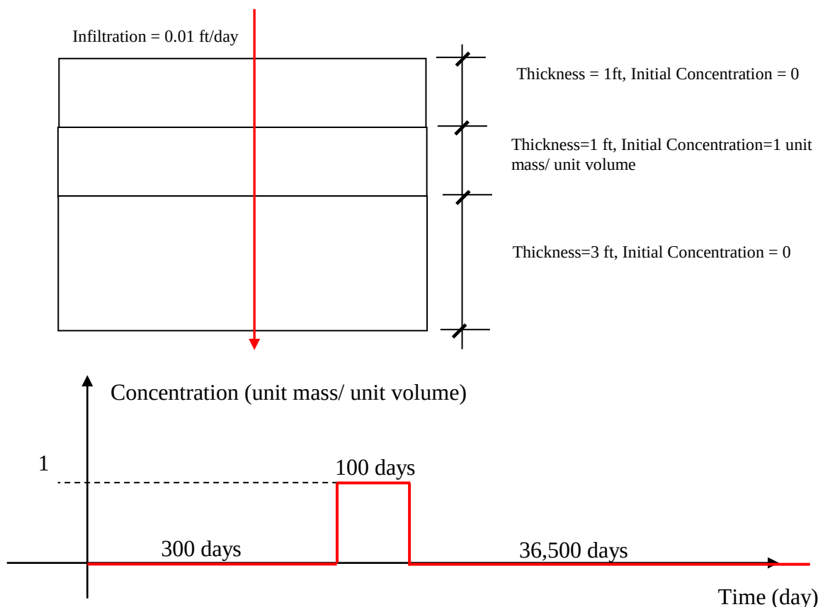
Figure G-7. Single-strip, Multiple-layer Source.
