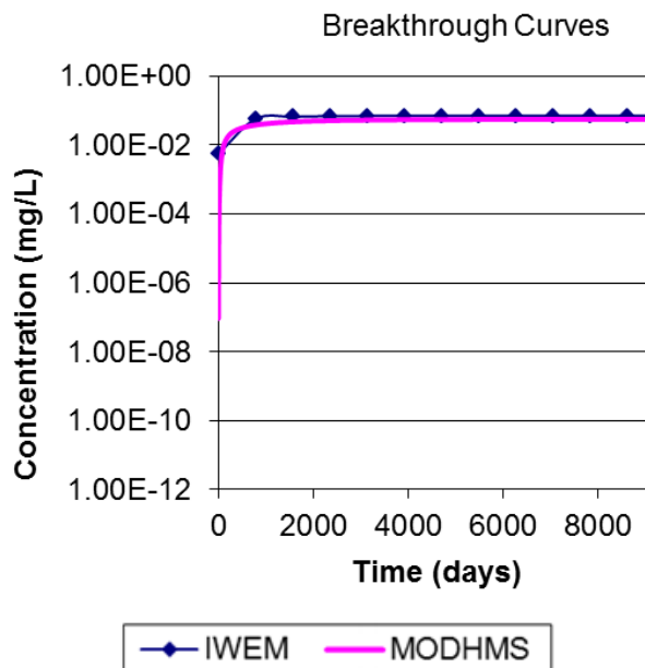
Figure G-13. Concentration at observation location 2 under single-strip, single-layer scenario with orthogonal flow.
