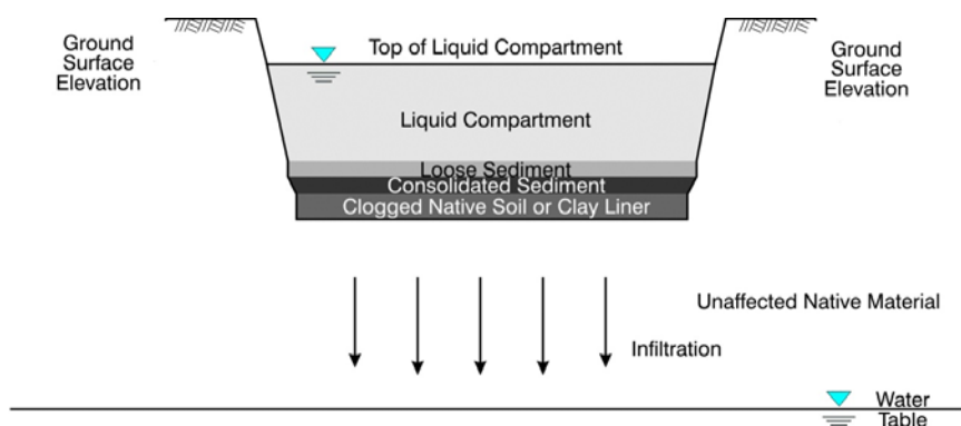
Figure 3-2. Surface impoundment infiltration module.
