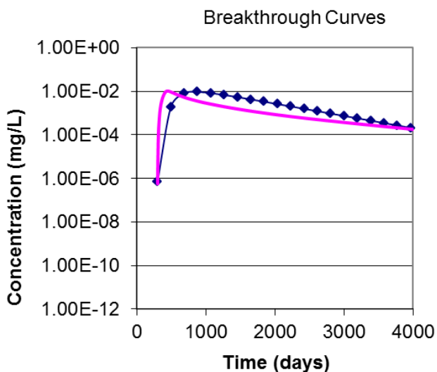
Figure G-19. Concentration at observation location 2 under single-strip, multiple-layer scenario with 45° flow.
