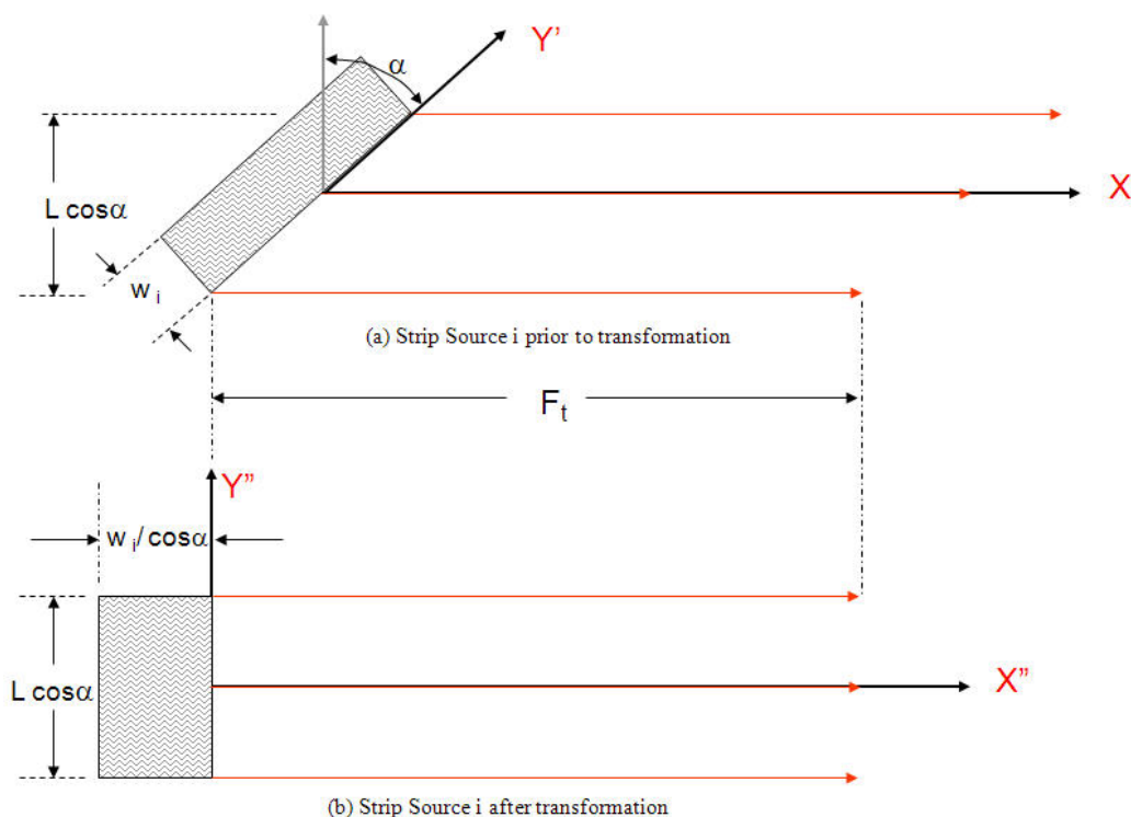
Figure F-2. Transformed orthogonal source for strip i .
