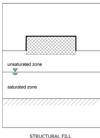
Figure 6-4. Structural fill modeled in IWEM.
