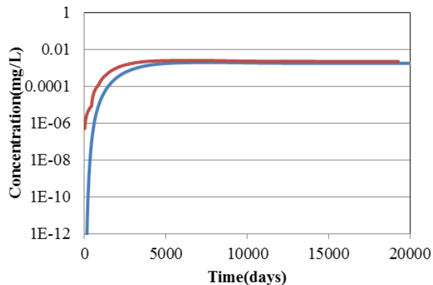
Figure G-27. Concentration at observation location 4.
