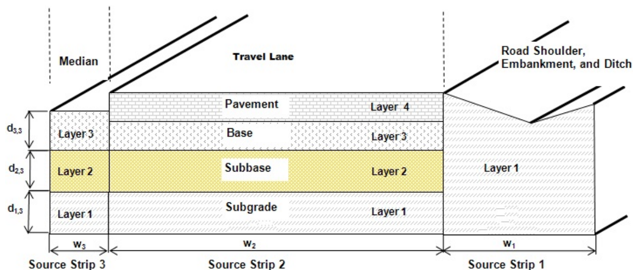
Figure C-4. An example of layering in roadway-source strips.
