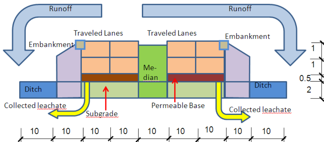
Figure G-10. Cross section of roadway segment in Case 4 with two symmetric drainage systems.
