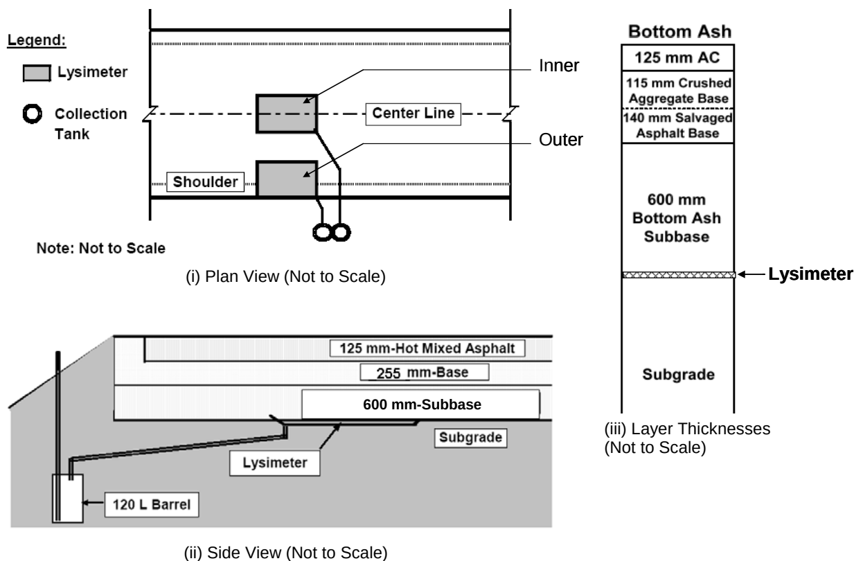
Figure E-4. Wisconsin State Highway 60 test section, experimental set up (from Li et al., 2005, and Sauer et al., 2005).
