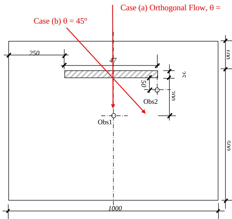
Figure G-6. Flow Angles
