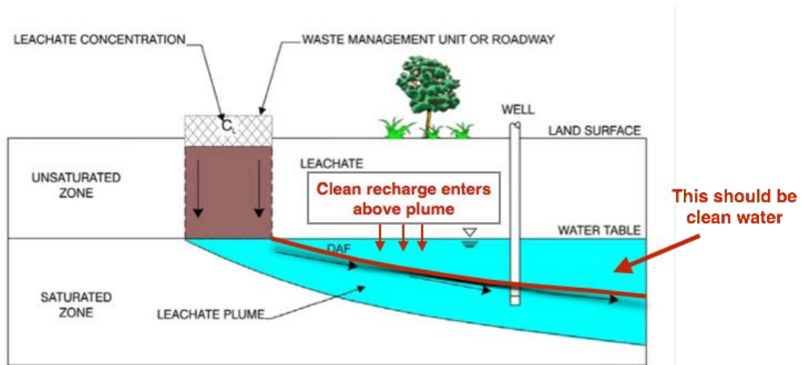
Figure ES-1 Conceptual cross-section view of the subsurface system simulated by EPACMTP.
