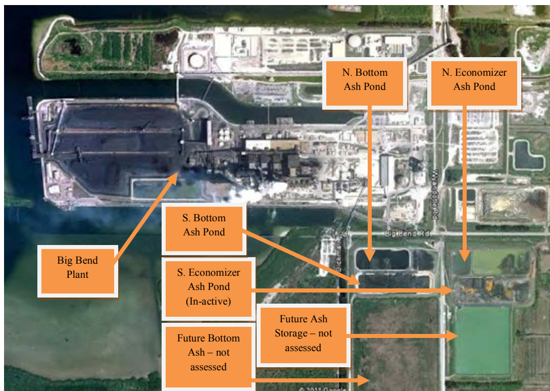
Figure 2.1b: Big Bend Plant Aerial View
